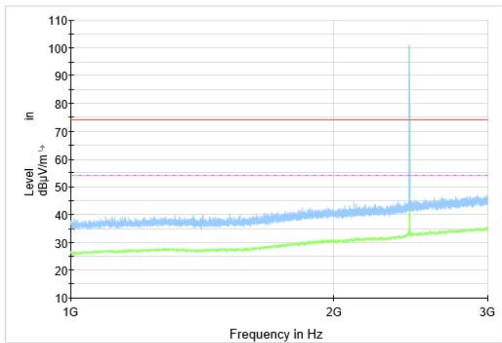
Fig. 44 Radiated Spurious Emission (GFSK, Ch39, 1 GHz ~3 GHz)
