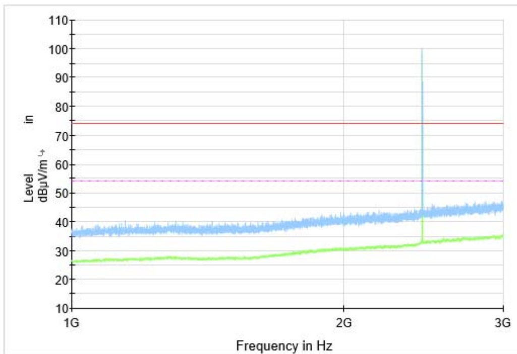
Fig. 60 Radiated Spurious Emission (8DPSK, Ch39, 1 GHz ~3 GHz)
