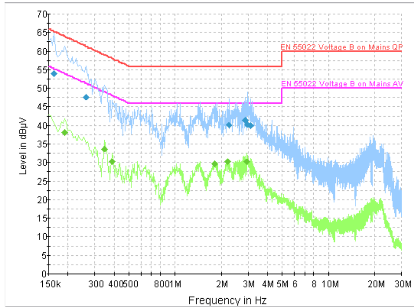
Fig.17 Conducted Emission
