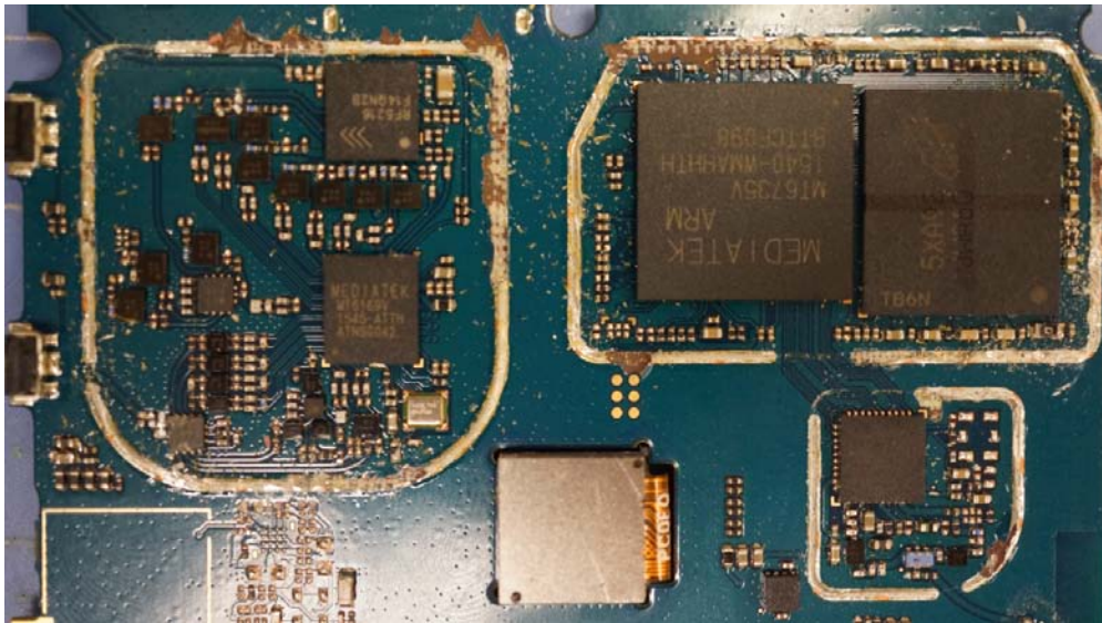
Mobile Phone Disassembly
