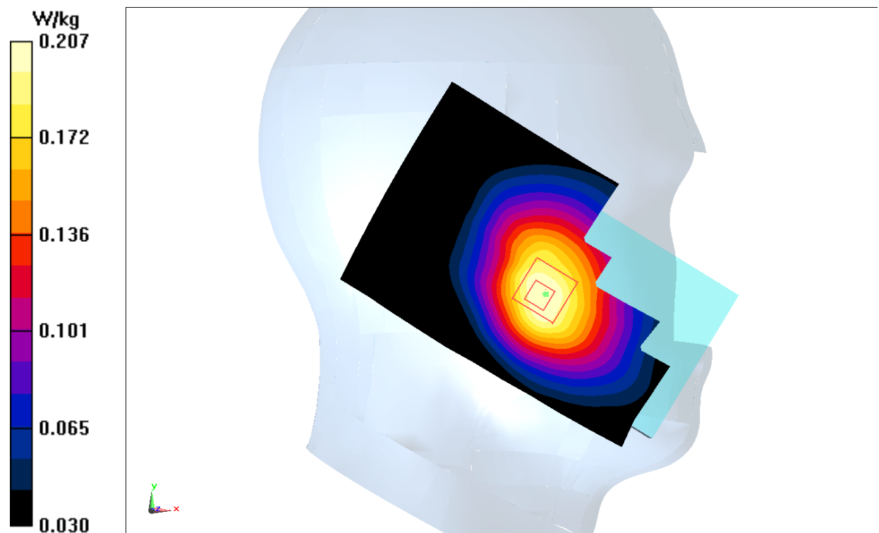
Fig.15 LTE Band 13
