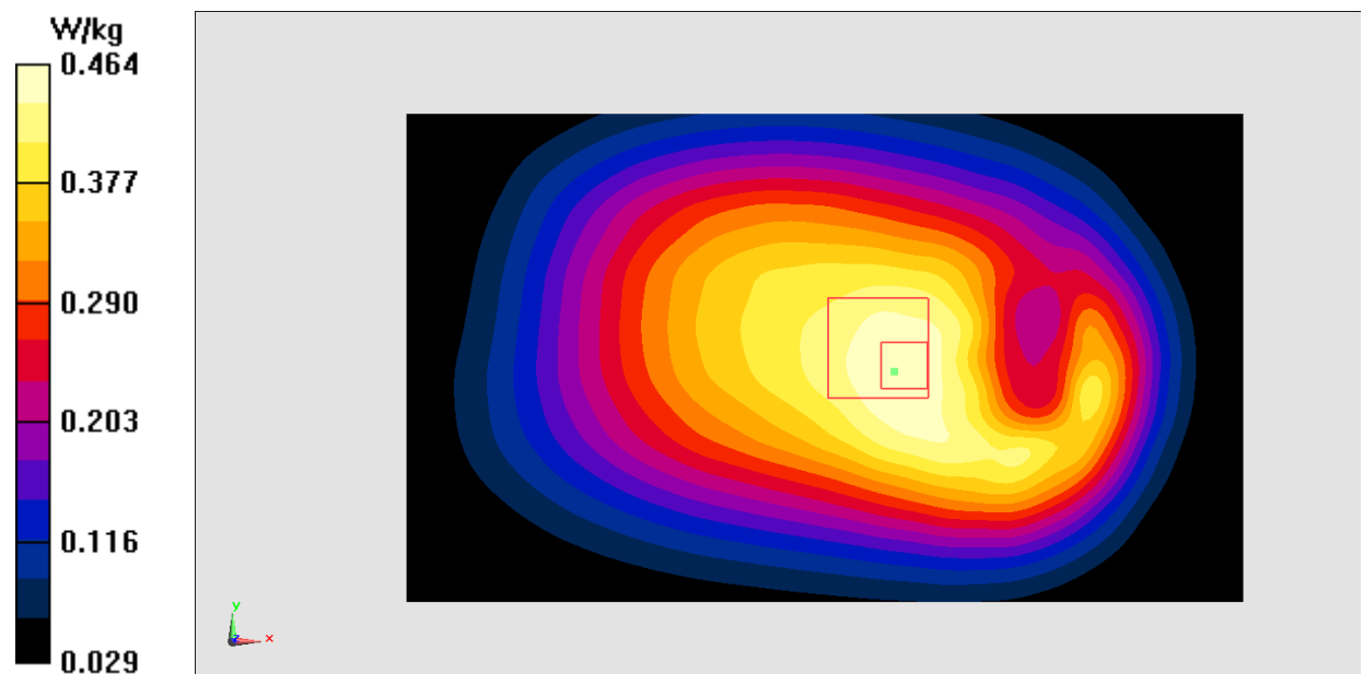
Fig.16 LTE Band 13
