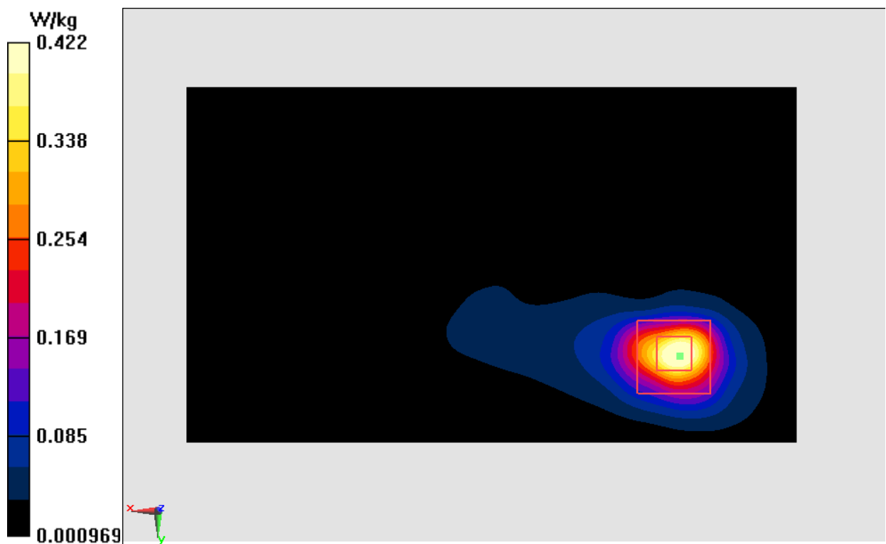
Fig.12 2450 MHz
