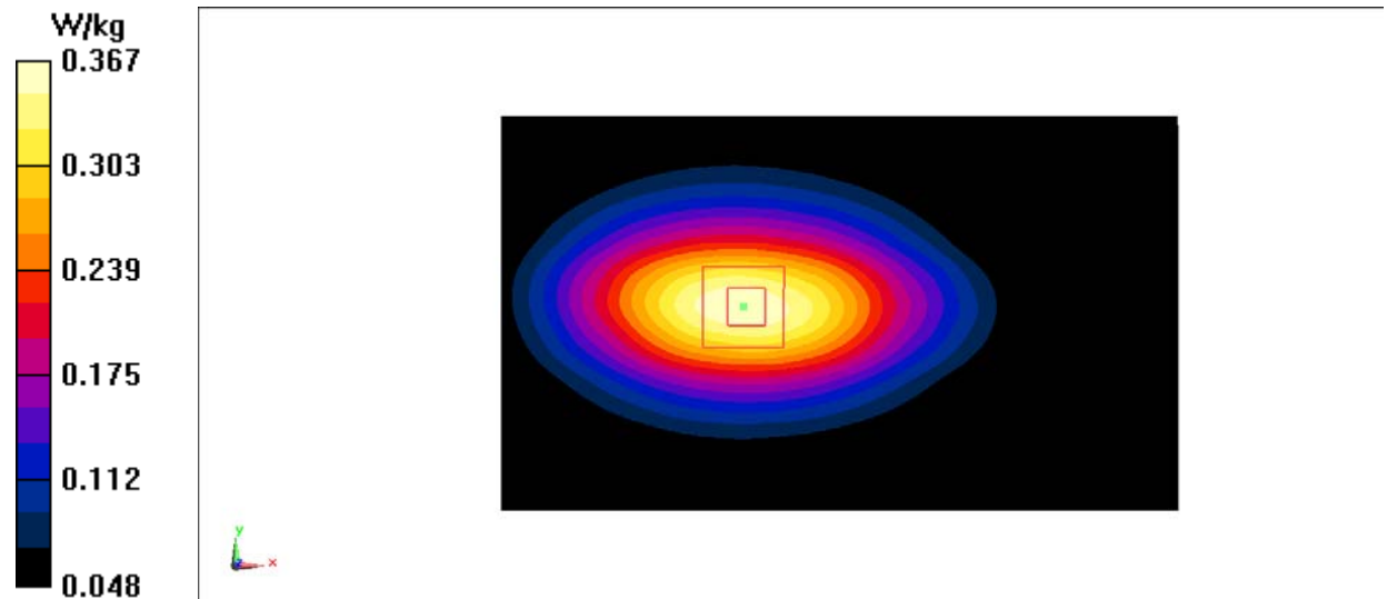
Fig.2 850 MHz
