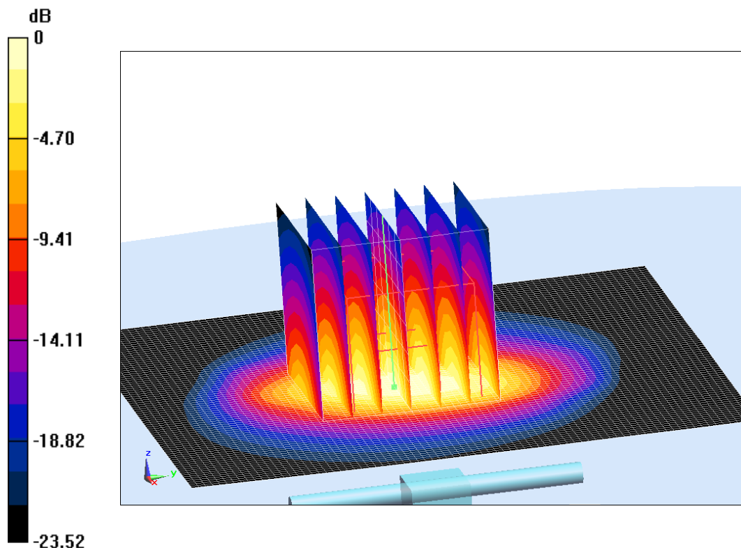
Fig.B.13 validation 2600 MHz 250mW
