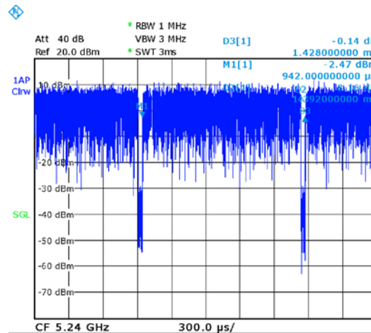
Picture 14.2 The plot of duty factor for WLAN-5G channel 48
