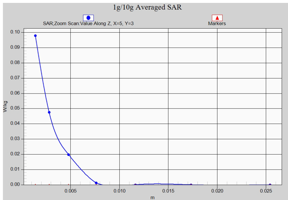
Fig. 13-1 Z-Scan at power reference point (5GHz)
