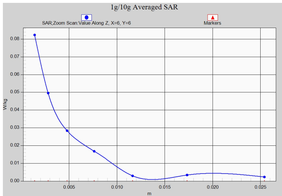
Fig. 14-1 Z-Scan at power reference point (5GHz)
