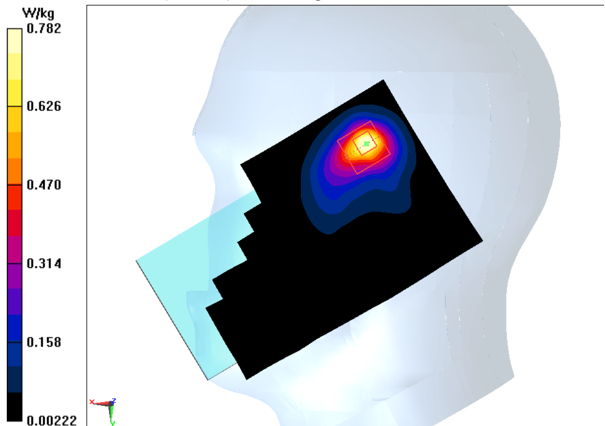
Fig.11 2450 MHz
