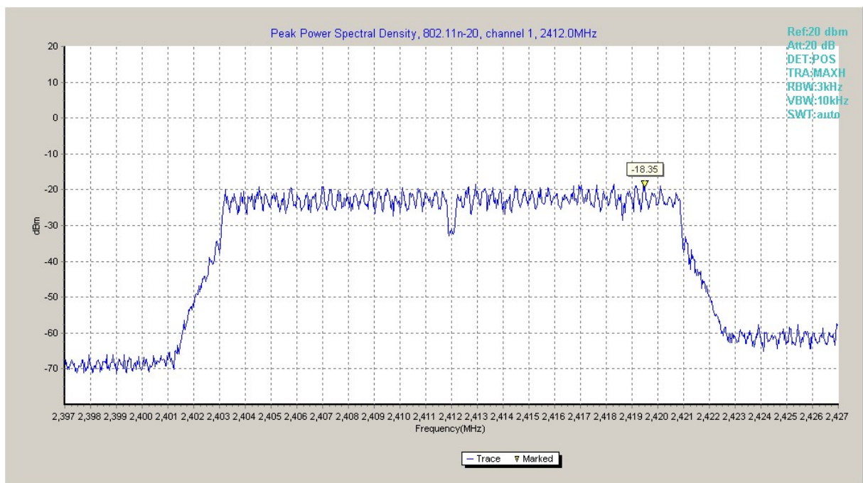
Fig.A.3.11 Power Spectral Density (802.11n-HT20, Ch 1)
