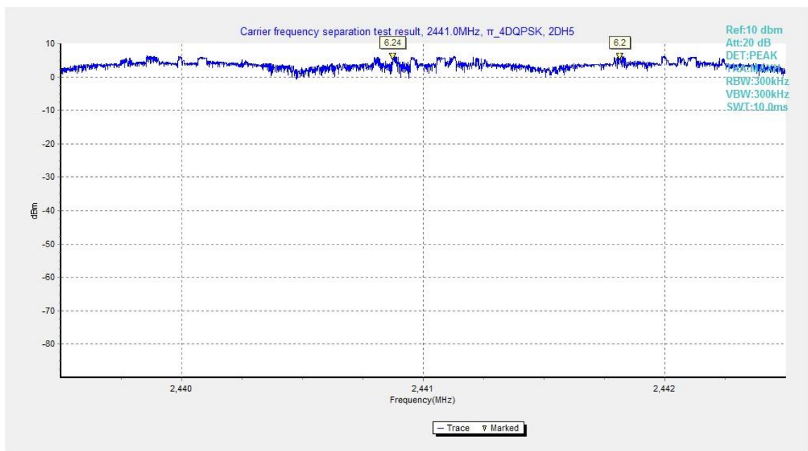
Fig.108. Carrier frequency separation measurement: \pi/4 DQPSK, Channel 39
