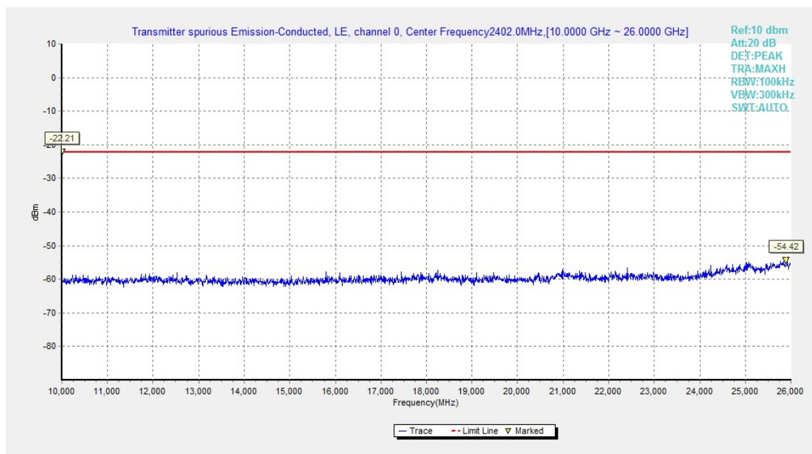
Fig.7. Transmitter Spurious Emission - Conducted: GFSK, 2402 MHz,10GHz - 26GHz
