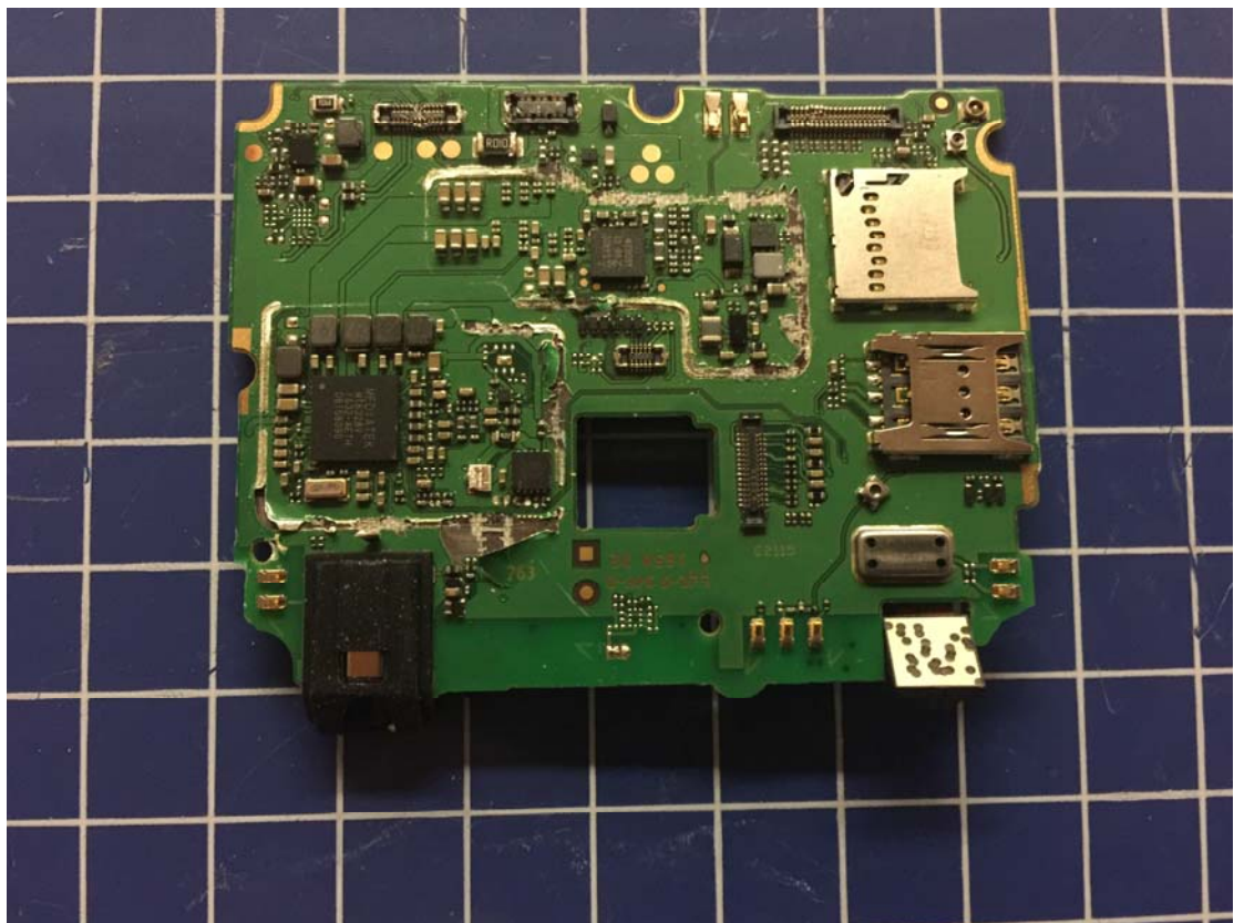
Pic A-6 Mobile phone Disassembly
