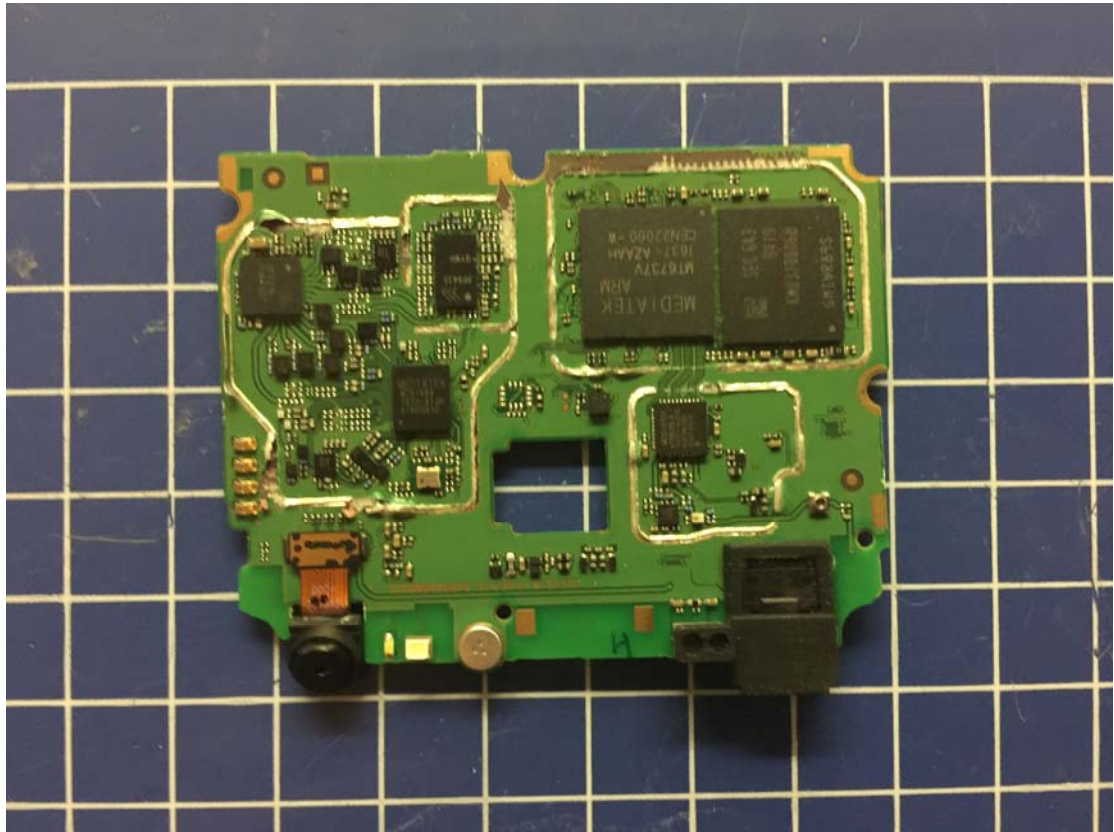
Pic A-5 Mobile phone Disassembly
