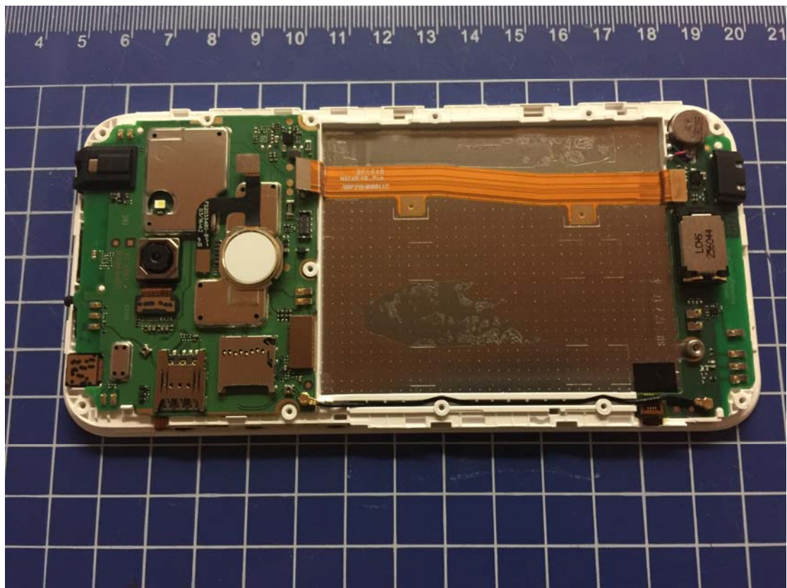
Pic A-3 Mobile phone Disassembly
