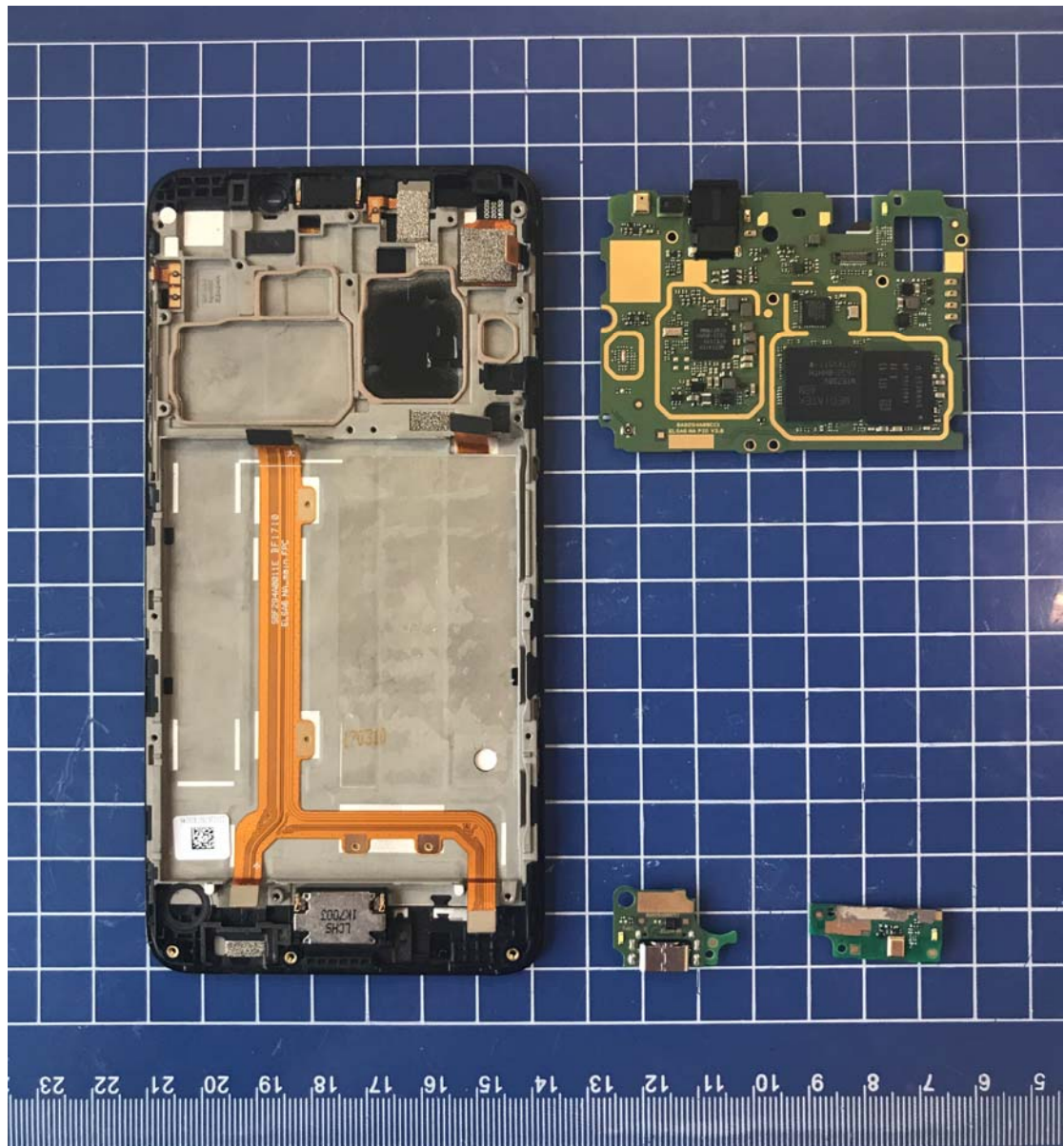
Mobile Phone Disassembly
