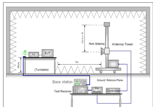
Figure 2. above 1GHz
