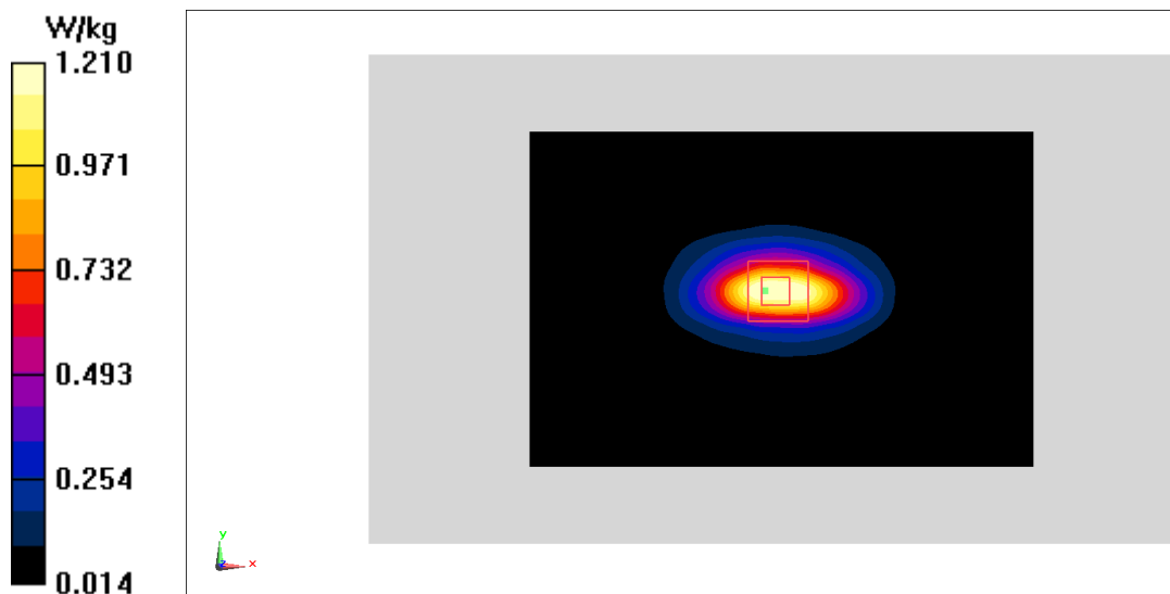
Fig.23 LTE Band66
