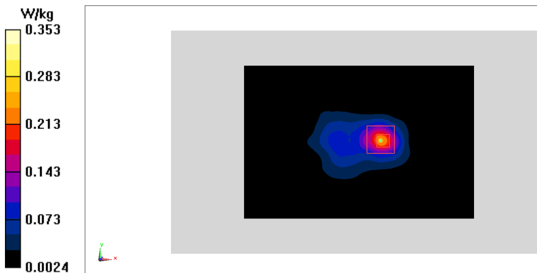
Fig.28 2450 MHz
