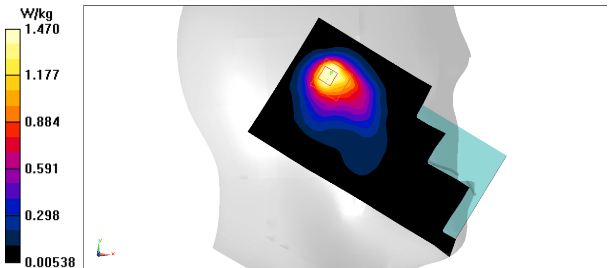
Fig.27 2450 MHz
