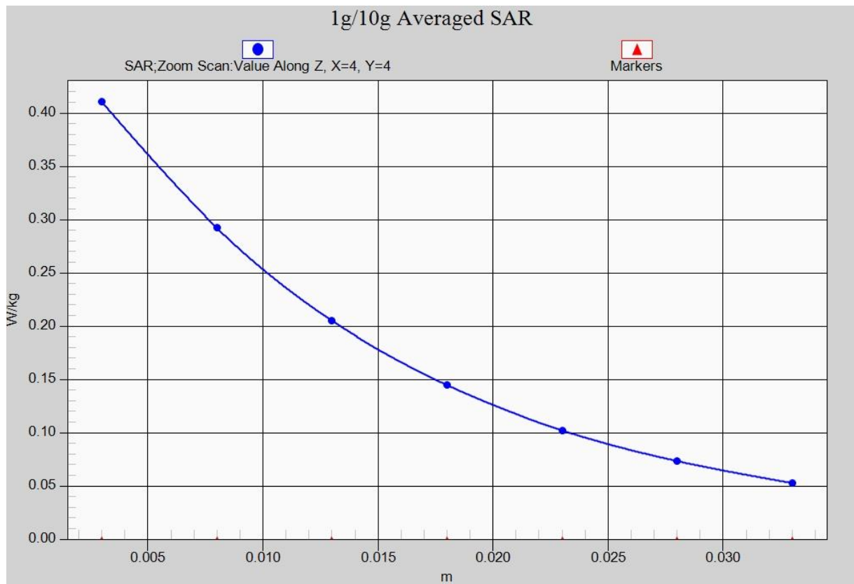
Fig. 22-1 Z-Scan at power reference point (LTE Band66)
