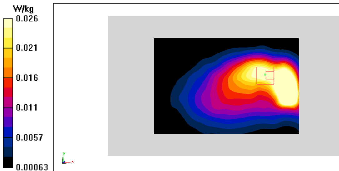
Fig.26 LTE Band71
