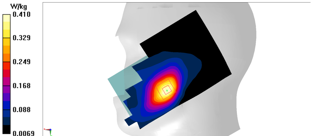
Fig.22 LTE Band66
