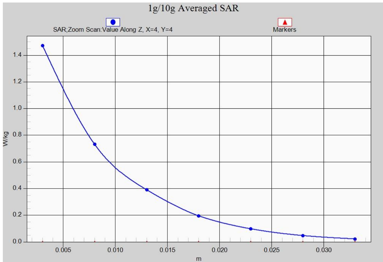
Fig. 27-1 Z-Scan at power reference point (2450 MHz)
