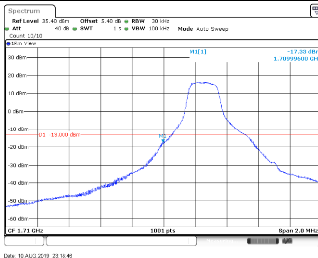
Band66_1.4MHz_QPSK_131979_6RB#0
