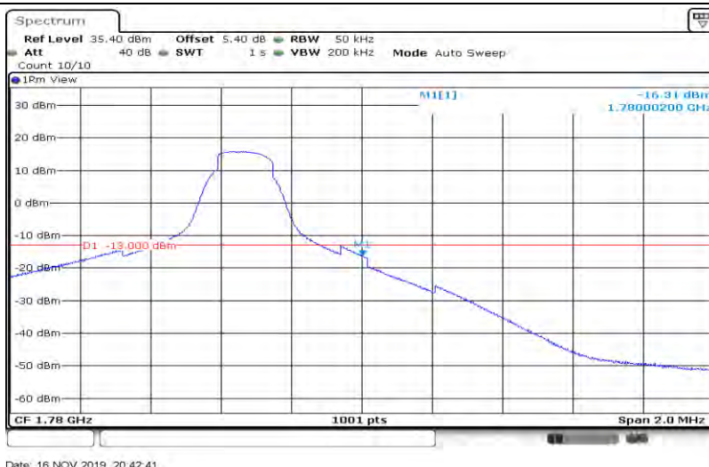
Band66-5MHz-QPSK-132647-25RB#0
