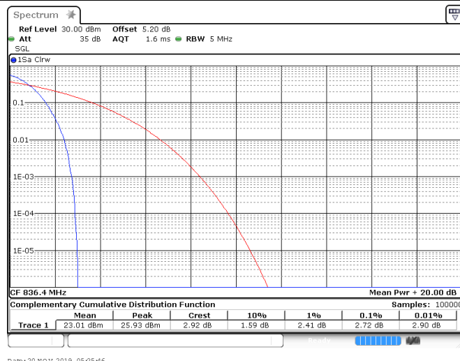
Band V_4233
