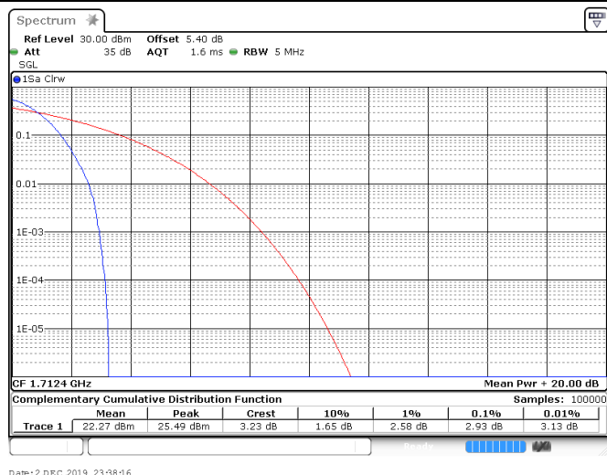
Band IV_1413
