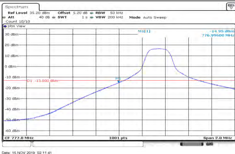
Band13-5MHz-16QAM-23205-25RB#0
