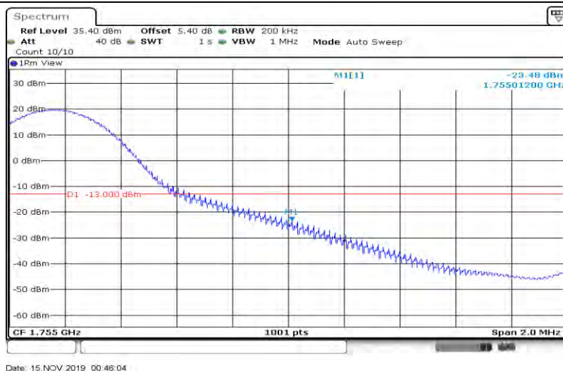
Band4-15MHz-16QAM-20325-75RB#0
