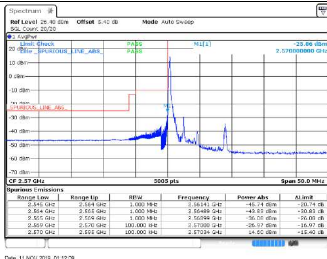
Band38_5MHz_16QAM_37775_25RB#0
