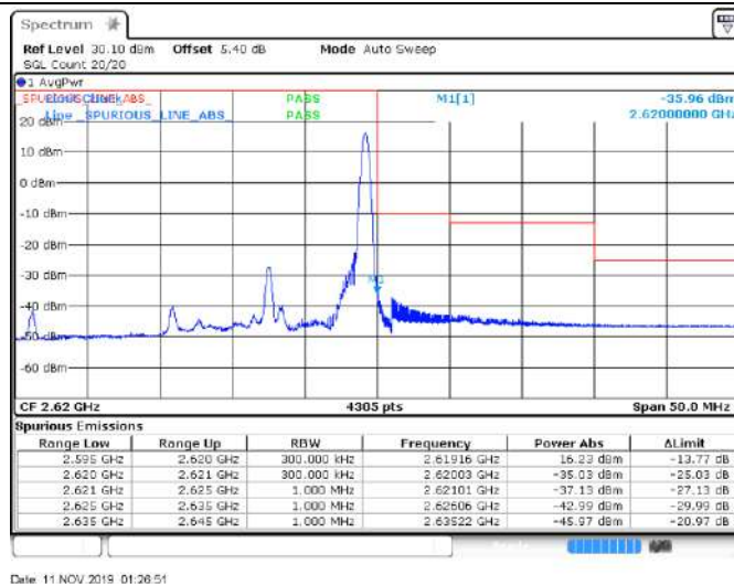
Band38_15MHz_QPSK_38175_75RB#0
