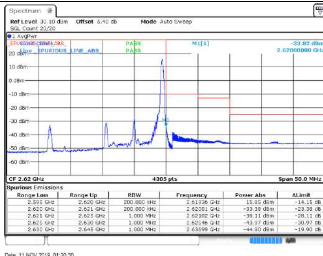
Band38_10MHz_16QAM_38200_50RB#0
