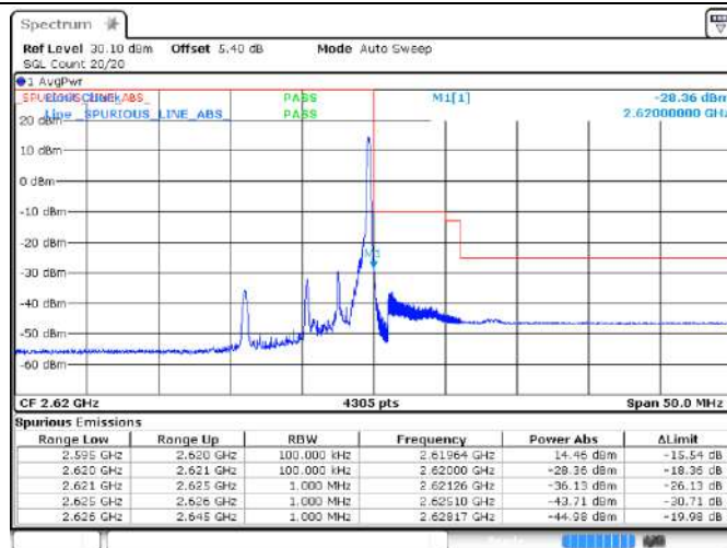
Band38_5MHz_16QAM_38225_25RB#0
