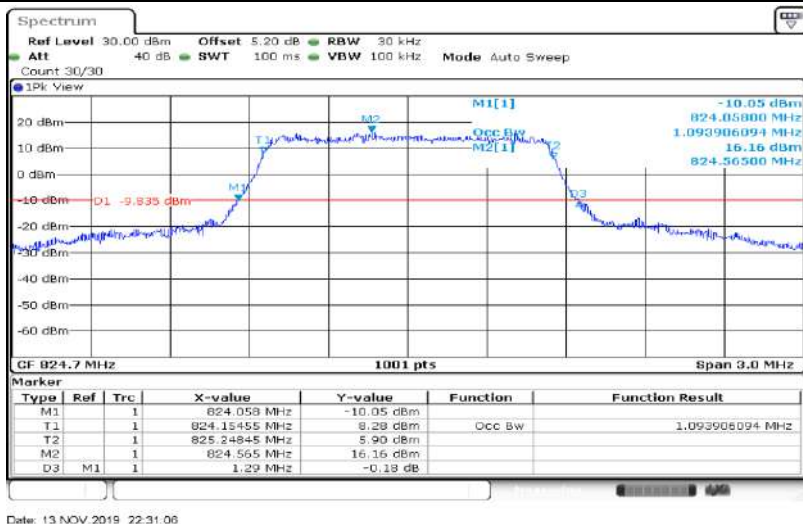
Band5-1.4MHz-16QAM-20525-6RB#0-1.097
