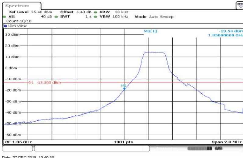
Band2-1.4MHz-16QAM-18607-6RB#0
