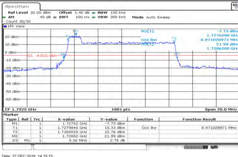
Band4-10MHz-QPSK-20350-50RB#0-8.971
