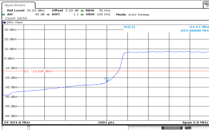
Band5-1.4MHz-16QAM-20407-6RB#0
