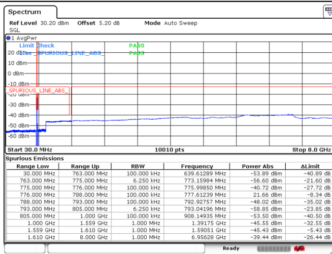
Band13-10MHz-QPSK-23230-1RB#0-Range1
