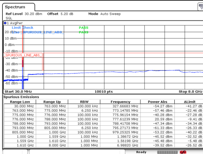
Band13-10MHz-16QAM-23230-1RB#0-Range1
