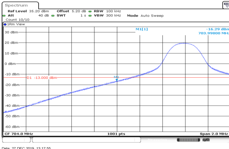
Band17-10MHz-16QAM-23780-50RB#0
