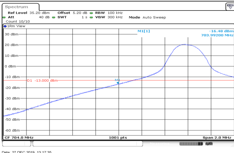
Band17-10MHz-QPSK-23780-50RB#0
