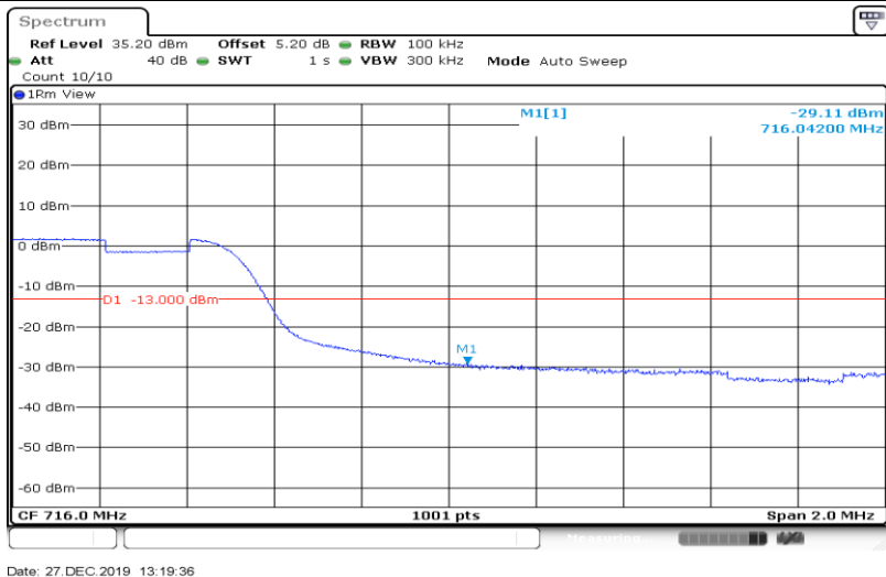
Band17-10MHz-16QAM-23780-1RB#0
