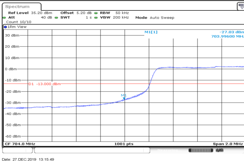
Band17-5MHz-16QAM-23825-1RB#24
