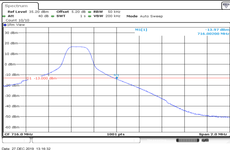
Band17-5MHz-16QAM-23825-25RB#0
