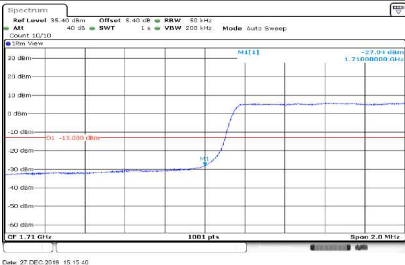
Band66-3MHz-QPSK-132657-1RB#14
