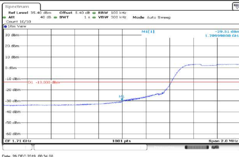
Band66-10MHz-16QAM-132622-1RB#49
