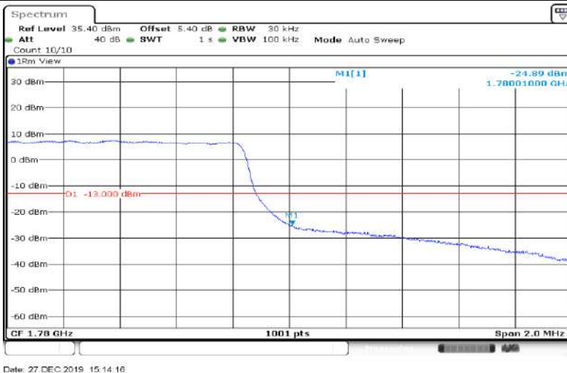
Band66-1.4MHz-16QAM-131979-1RB#0
