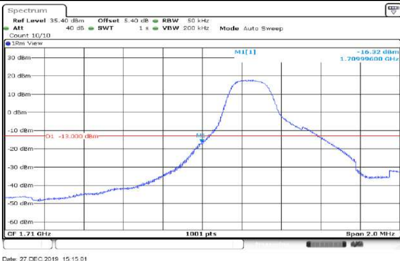
Band66-3MHz-QPSK-131987-15RB#0
