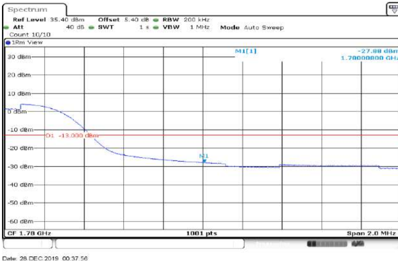
Band66-15MHz-16QAM-132047-1RB#0
