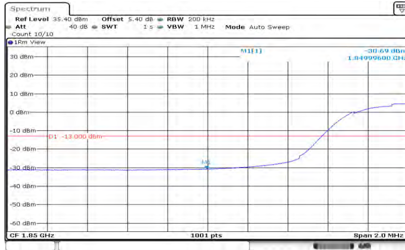
Band2-15MHz-16QAM-18675-75RB#0
