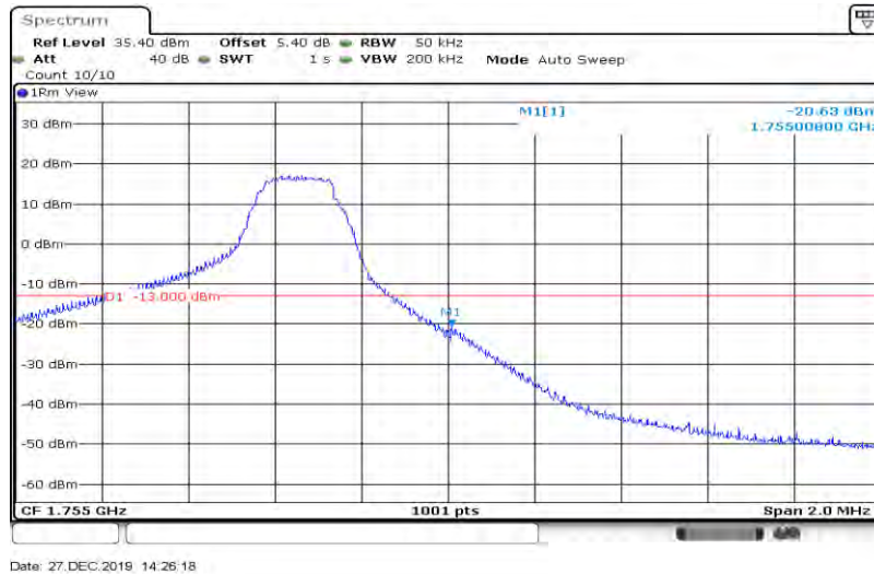
Band4-5MHz-16QAM-20375-25RB#0
