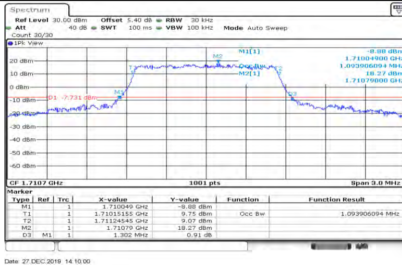
Band4-1.4MHz-QPSK-20175-6RB#0-1.085
