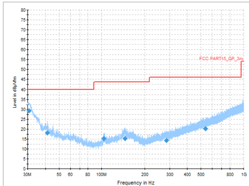
Figure A.9 Radiated Emission (Set.1, Charging and LTE Band 14 idle, 30MHz to 1GHz) Final_Result
