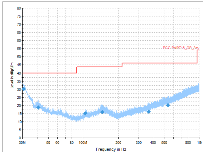
Figure A.7 Radiated Emission (Set.1, Charging and LTE Band 12 idle, 30MHz to 1GHz) Final_Result
