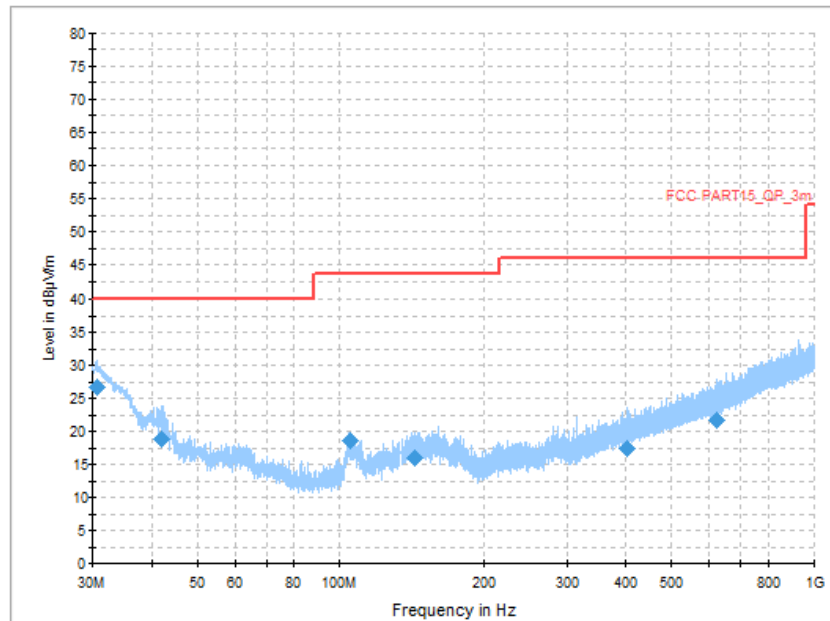
Figure A.1 Radiated Emission (Set.1, Charging and GSM850MHz idle, 30MHz to 1GHz) Final_Result
