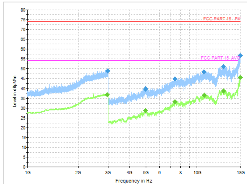
Figure A.6 Radiated Emission (Set.1, Charging and LTE Band 5 idle , 1GHz to 18GHz) Final_Results_PK
