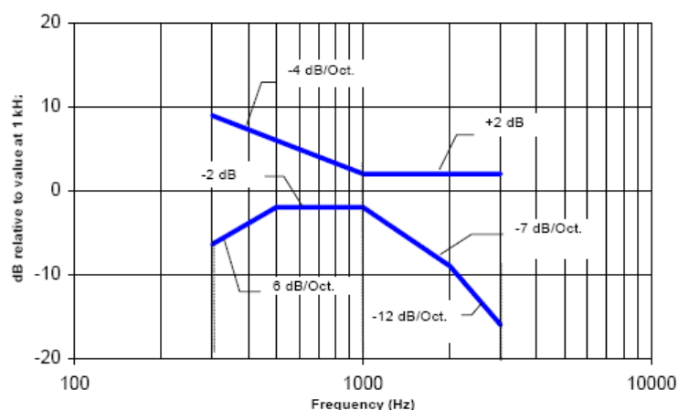
Figure 7.2—Magnetic field frequency response for WDs with a field that exceeds -
