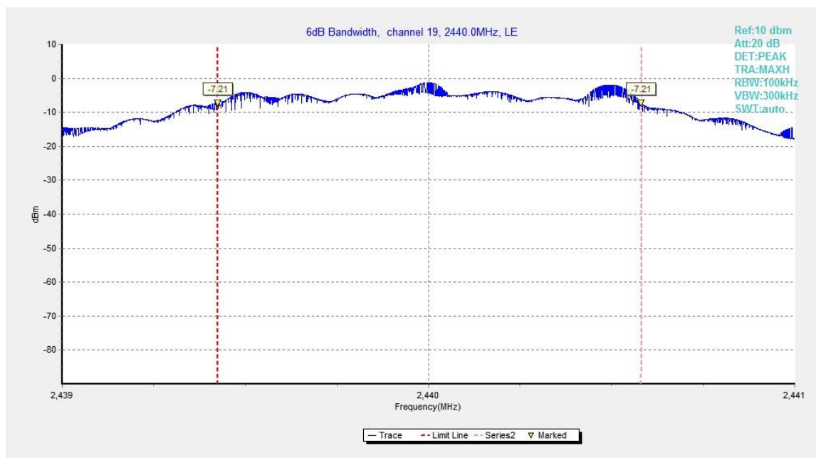
Fig.23. 6dB Bandwidth: GFSK, 2440 MHz
