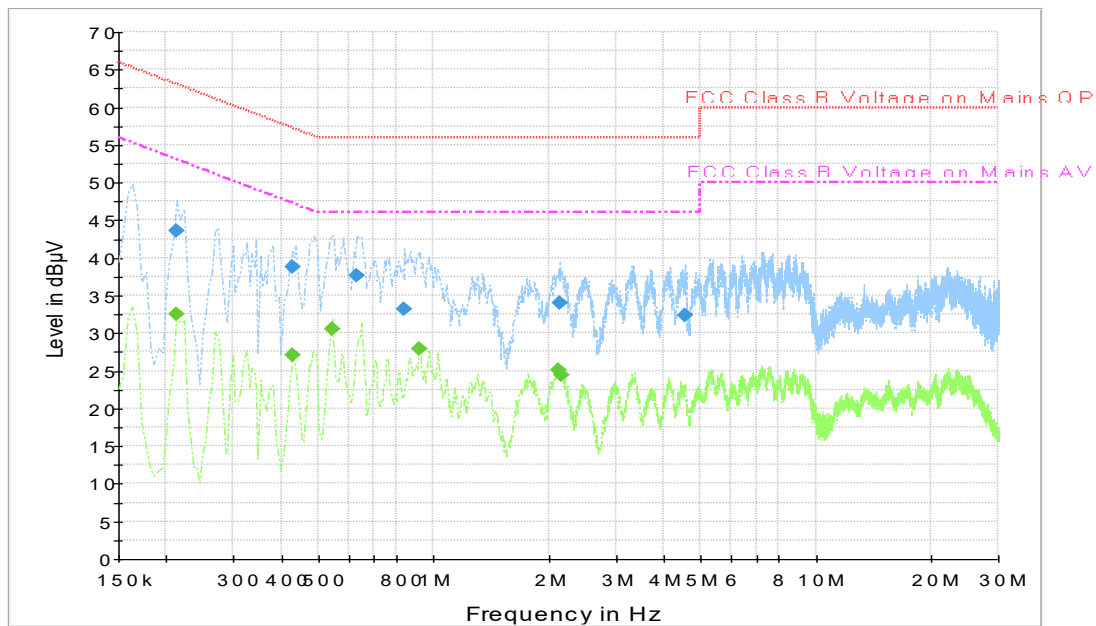
Fig.A.9.1 AC Powerline Conducted Emission-BLE4.0-traffic
