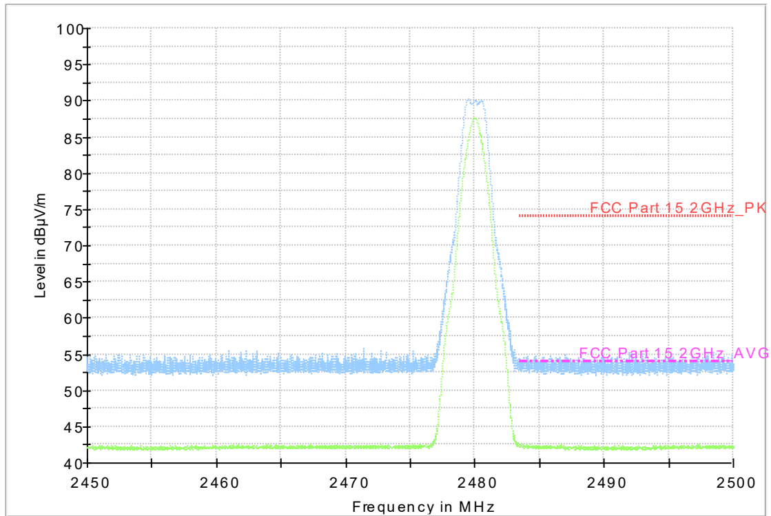
Fig.6. Frequency Band Edges: GFSK, 2480 MHz, BLE 5.0, Hopping Off , 2.45 GHz - 2.50GHz
