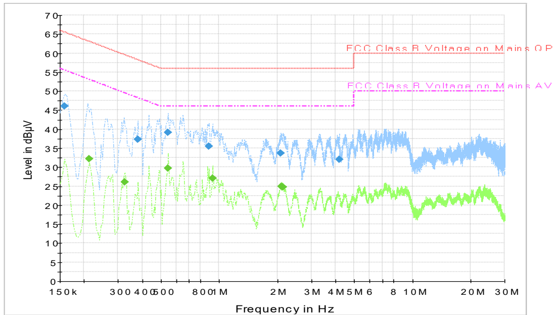
Fig.A.9.2 AC Powerline Conducted Emission BLE4.0-Idle
