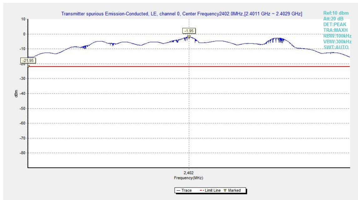
Fig.7. Transmitter Spurious Emission - Conducted: GFSK, 2402MHz
