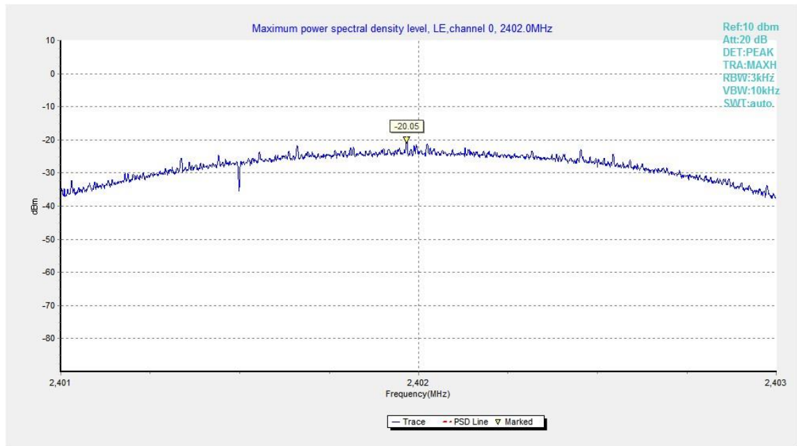
Fig.25. Maximum Power Spectral Density Level Function: GFSK, 2402 MHz
