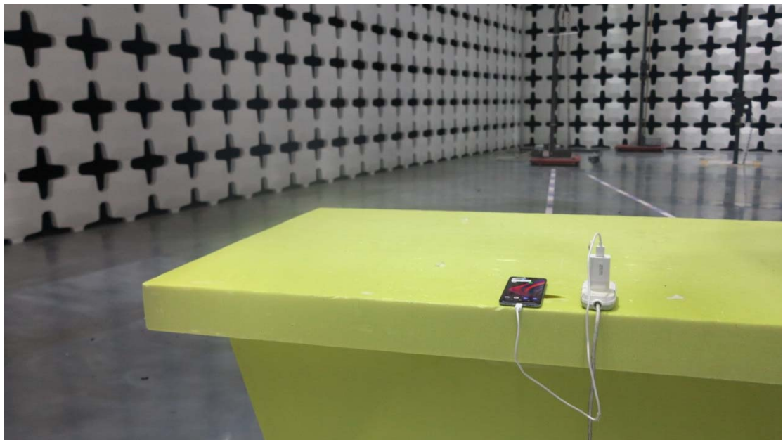
15B USB 30MHz-1GHz
