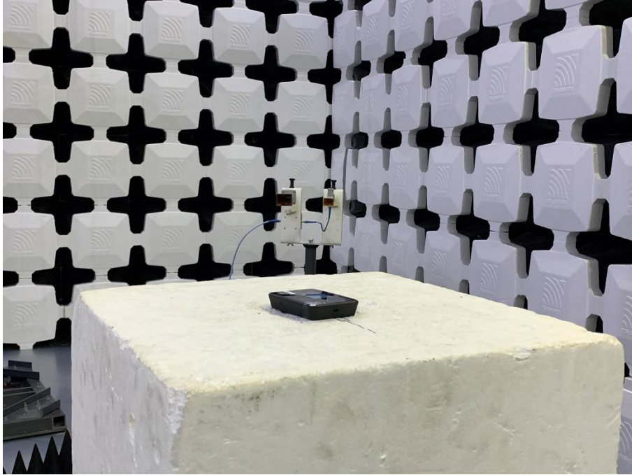
7. Radiated Emissions (Part 22/24/27, 26.5GHz -40GHz)
