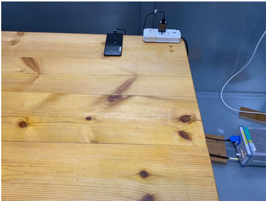
8. Conducted Emission (Part 15B, Charger+MP4/GNSS/ Camera /GSM idle/WCDMA idle/LTE idle)
