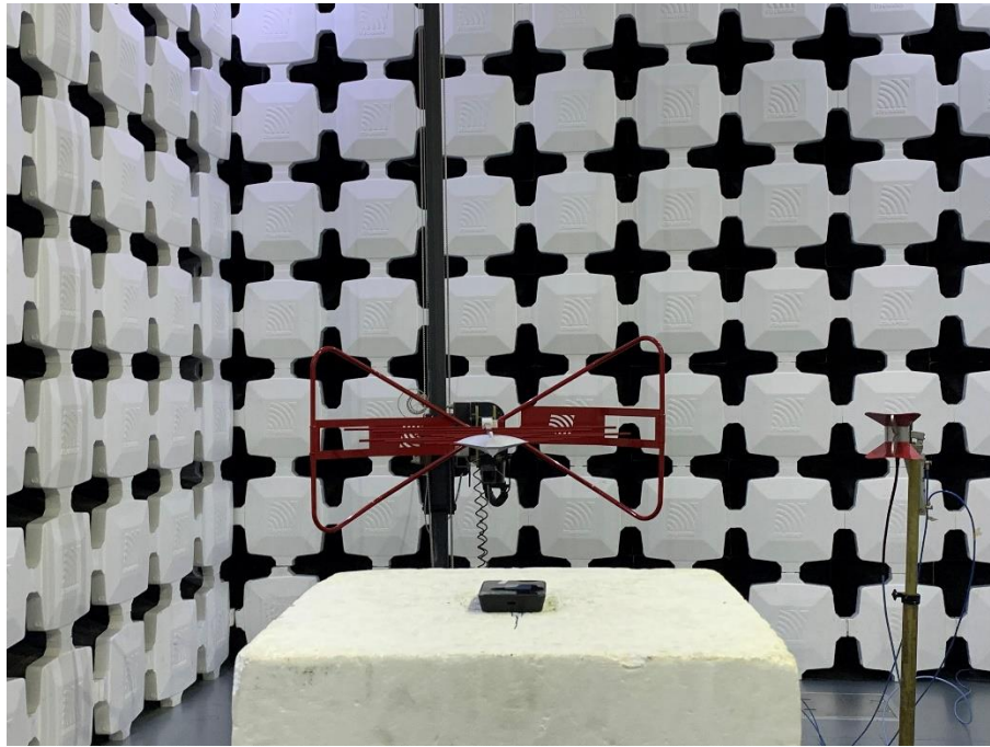
5. Radiated Emissions (Part 22/24/27,30MHz-18GHz)
