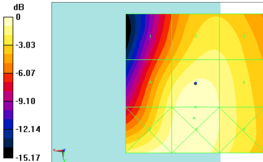
Fig B.3 HAC RF E-Field LTE Band41 PC2 16QAM CH40620
