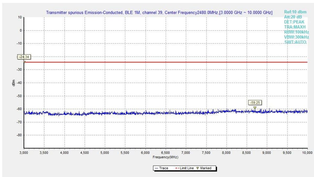
Fig.25 Conducted Spurious Emission (Ch39, 3 GHz-10 GHz), LE 1M
