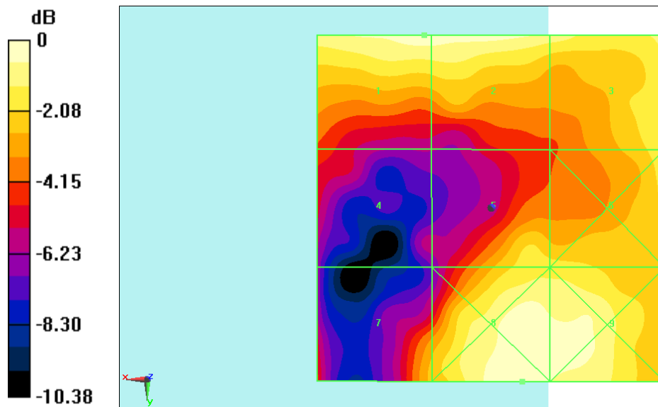
Fig B.4 HAC RF E-Field LTE Band41 16QAM PC3
