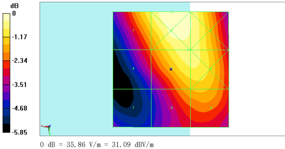
Fig B.2 HAC RF E-Field GSM1900
