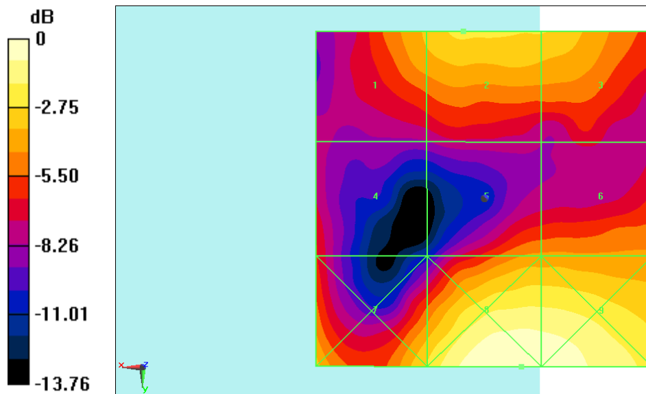
Fig B.3 HAC RF E-Field LTE Band41 QPSK PC2
