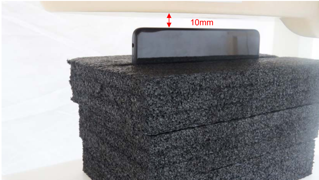
Picture 9: Left Edge, the distance from handset to the bottom of the Phantom is 10mm
