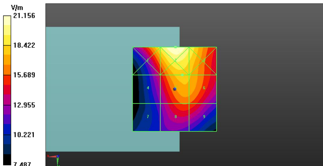
Fig A.5 HAC RF E-Field LTE-Band 41
