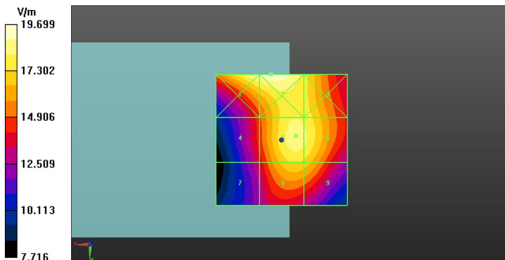
Fig A.2 HAC RF E-Field LTE-Band 41
