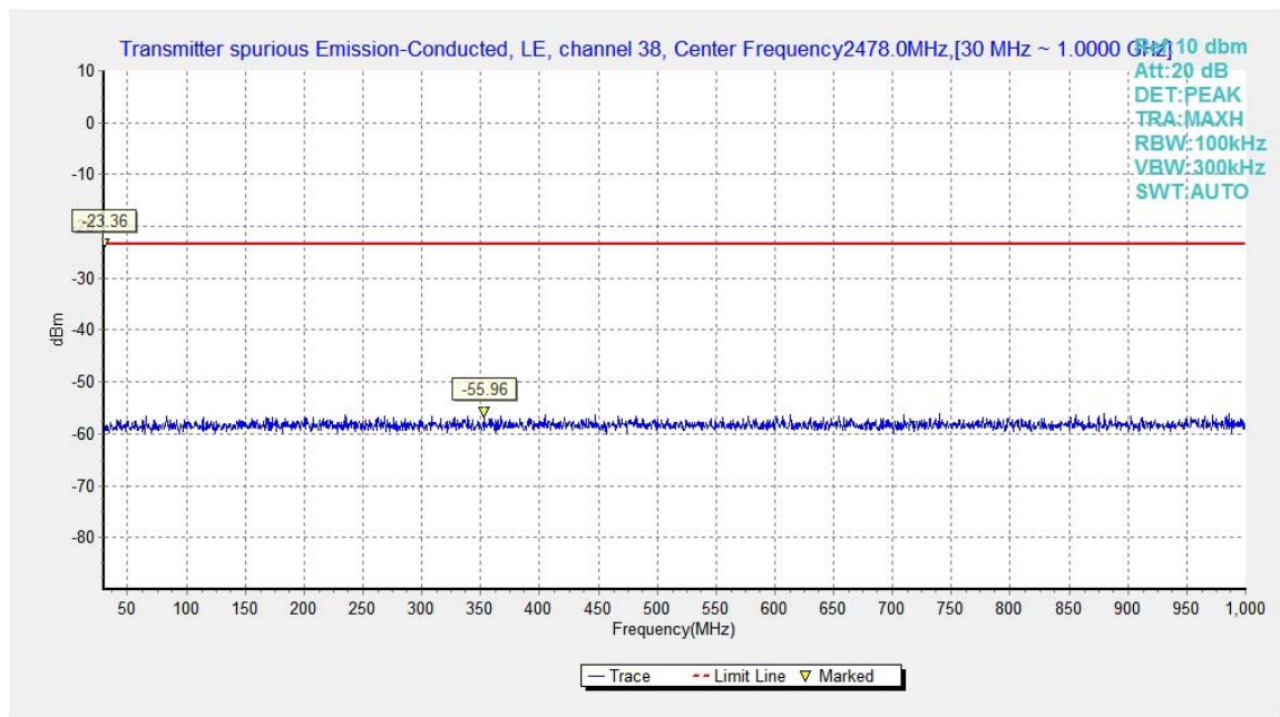
Fig.16. Transmitter Spurious Emission - Conducted: GFSK, 2478 MHz, 30MHz - 1GHz
