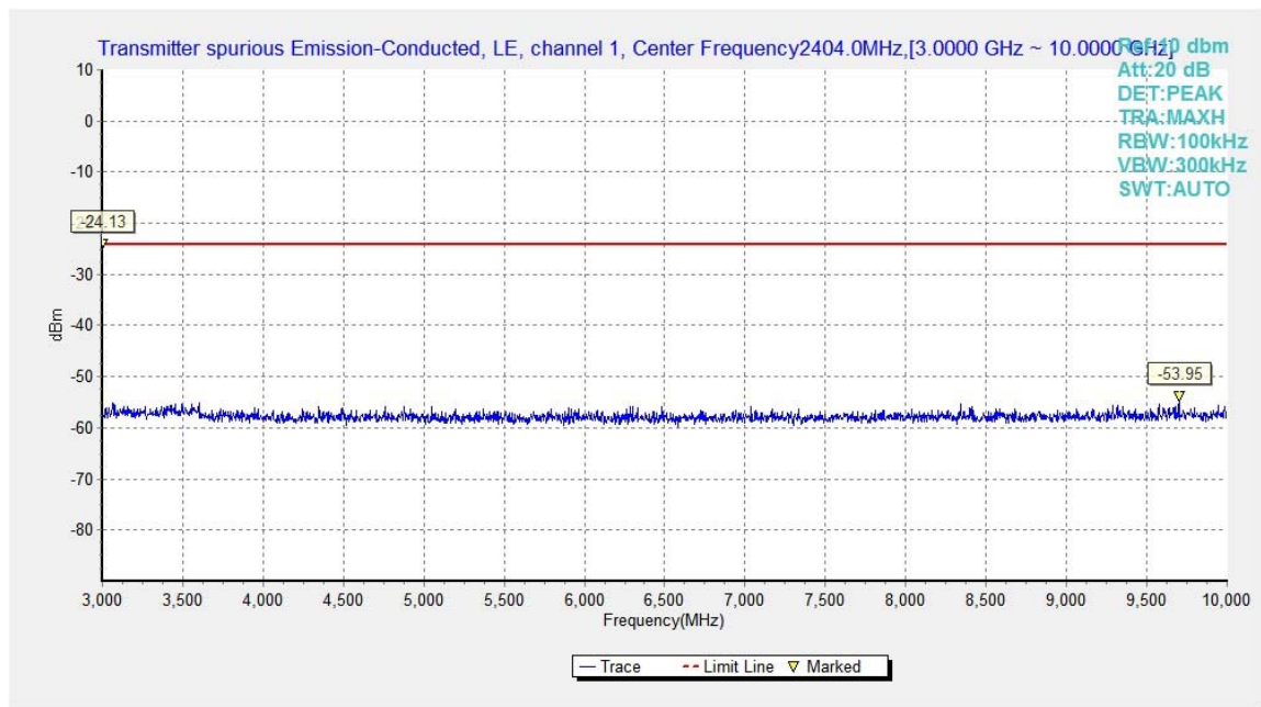
Fig.8. Transmitter Spurious Emission - Conducted: GFSK, 2404 MHz, 3GHz - 10GHz
