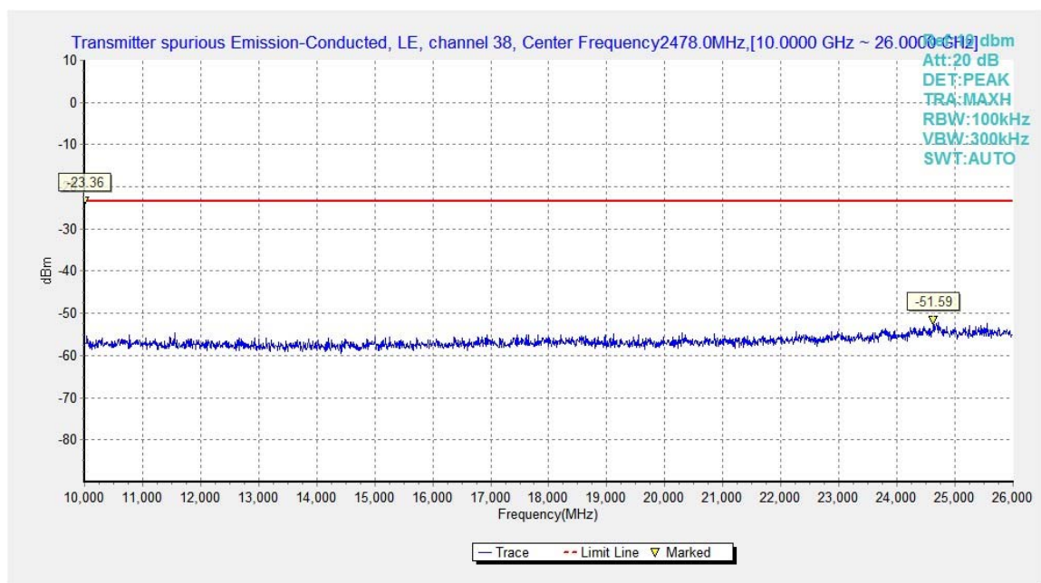
Fig.19. Transmitter Spurious Emission - Conducted: GFSK, 2478 MHz, 10GHz - 26GHz
