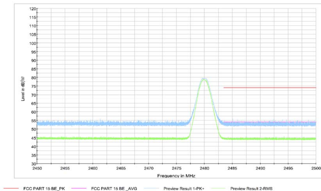
Fig.4. Frequency Band Edges: GFSK, 2480 MHz, Hopping Off, 2.45 GHz - 2.50GHz
