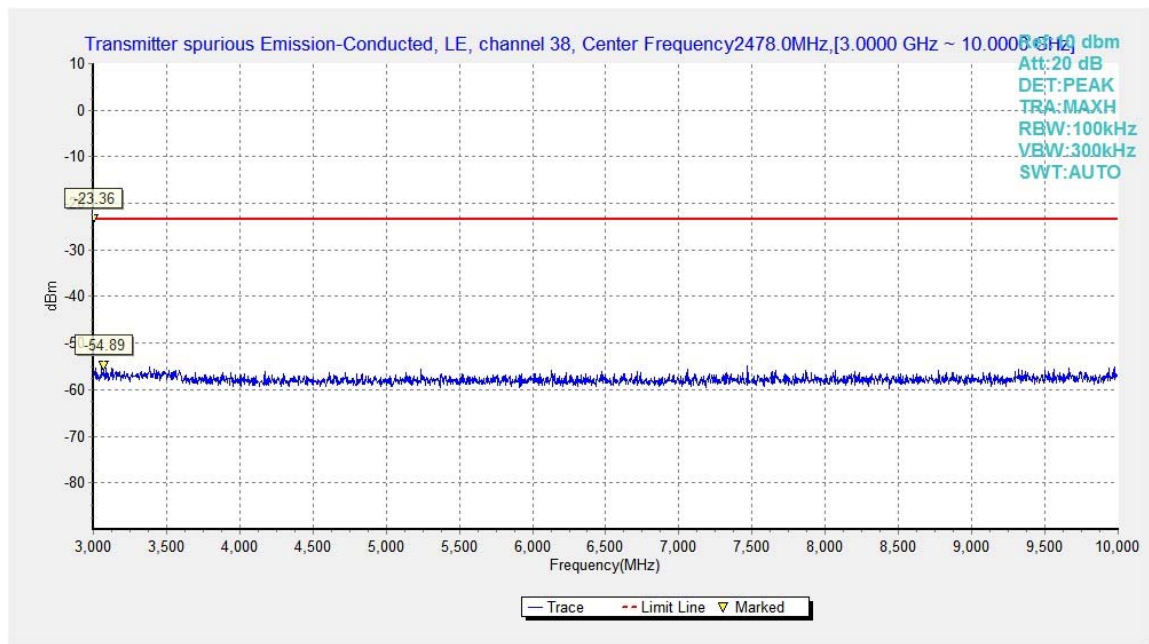
Fig.18. Transmitter Spurious Emission - Conducted: GFSK, 2478 MHz, 3GHz - 10GHz
