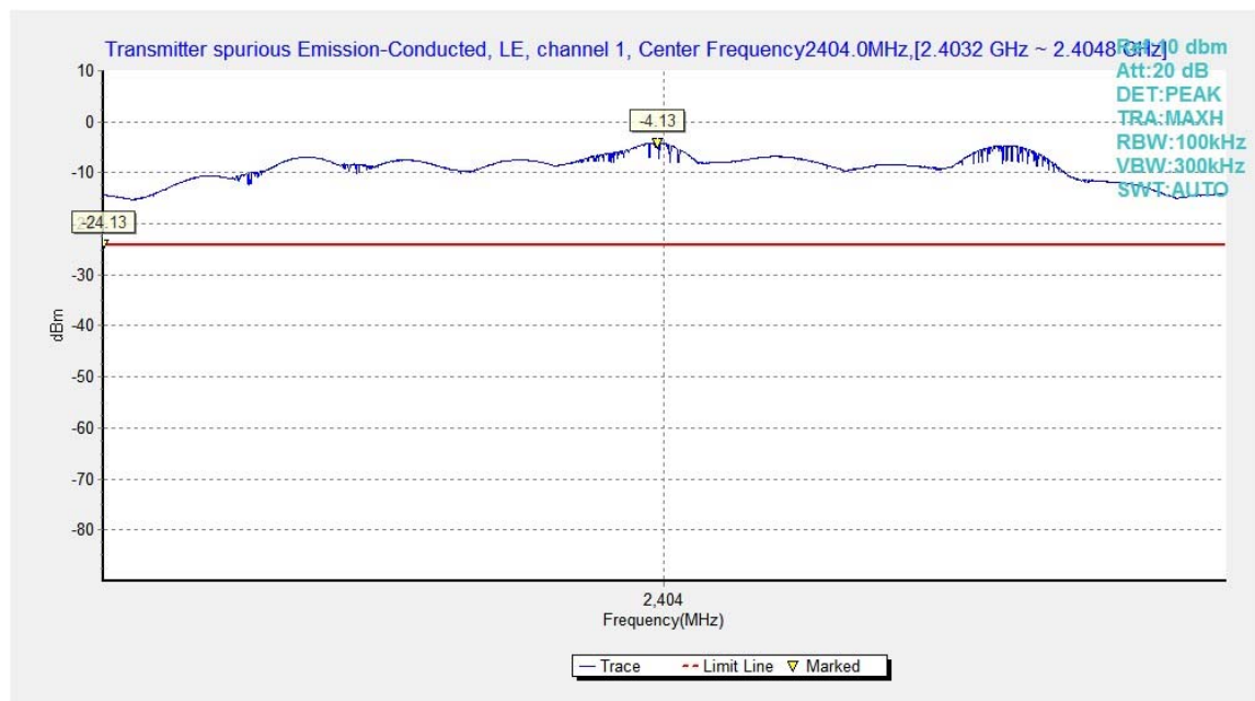
Fig.5. Transmitter Spurious Emission - Conducted: GFSK, 2404MHz
