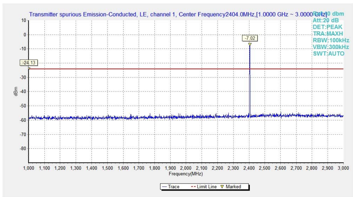
Fig.7. Transmitter Spurious Emission - Conducted: GFSK, 2404 MHz, 1GHz - 3GHz
