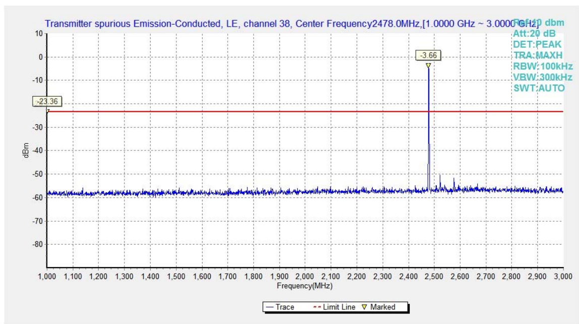
Fig.17. Transmitter Spurious Emission - Conducted: GFSK, 2478 MHz, 1GHz - 3GHz
