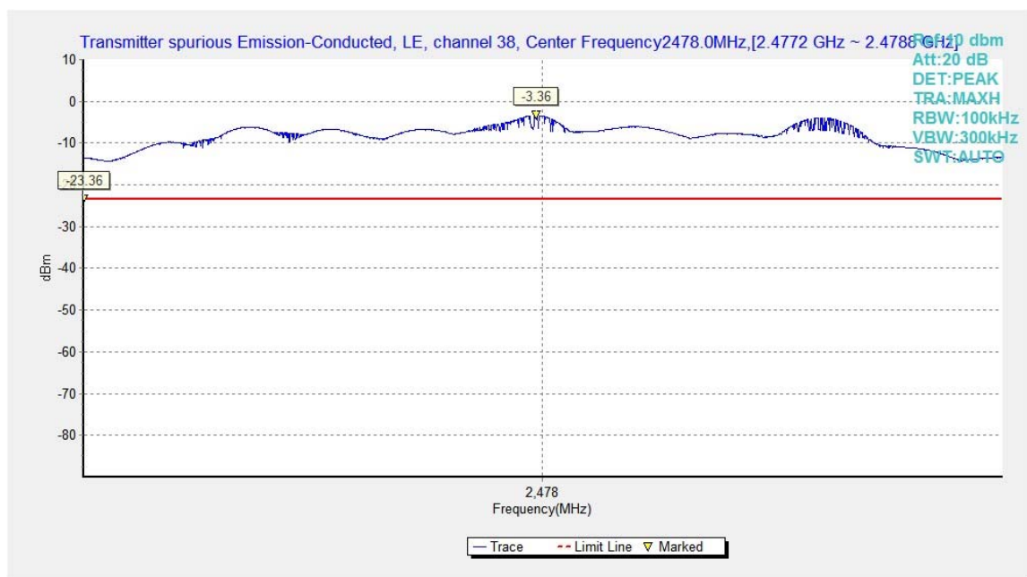
Fig.15. Transmitter Spurious Emission - Conducted: GFSK, 2478 MHz
