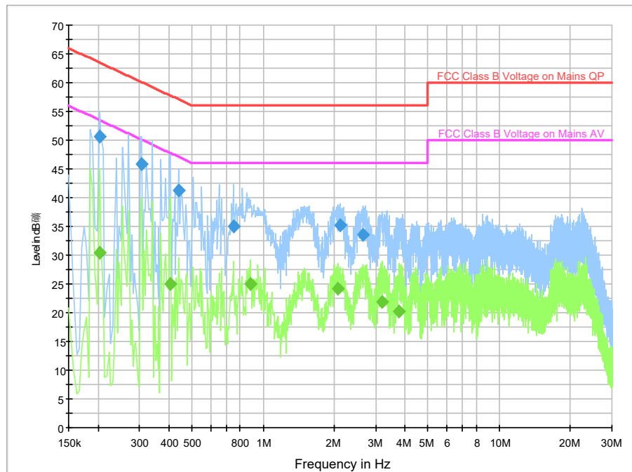
Fig.B.9.2 AC Powerline Conducted Emission-Idle
