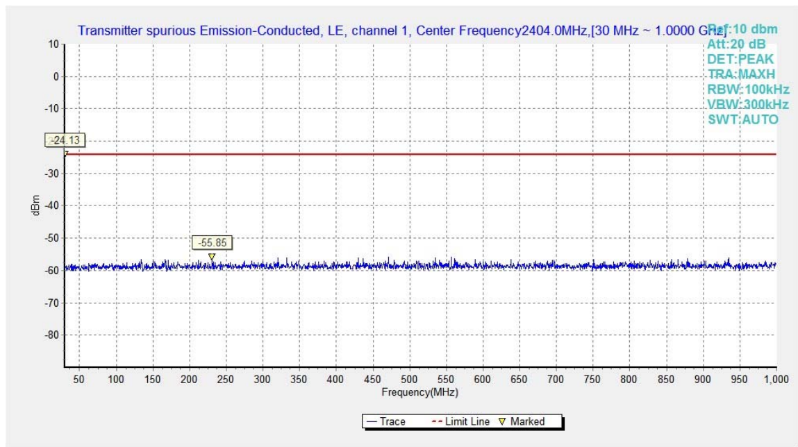
Fig.6. Transmitter Spurious Emission - Conducted: GFSK, 2404 MHz, 30MHz - 1GHz
