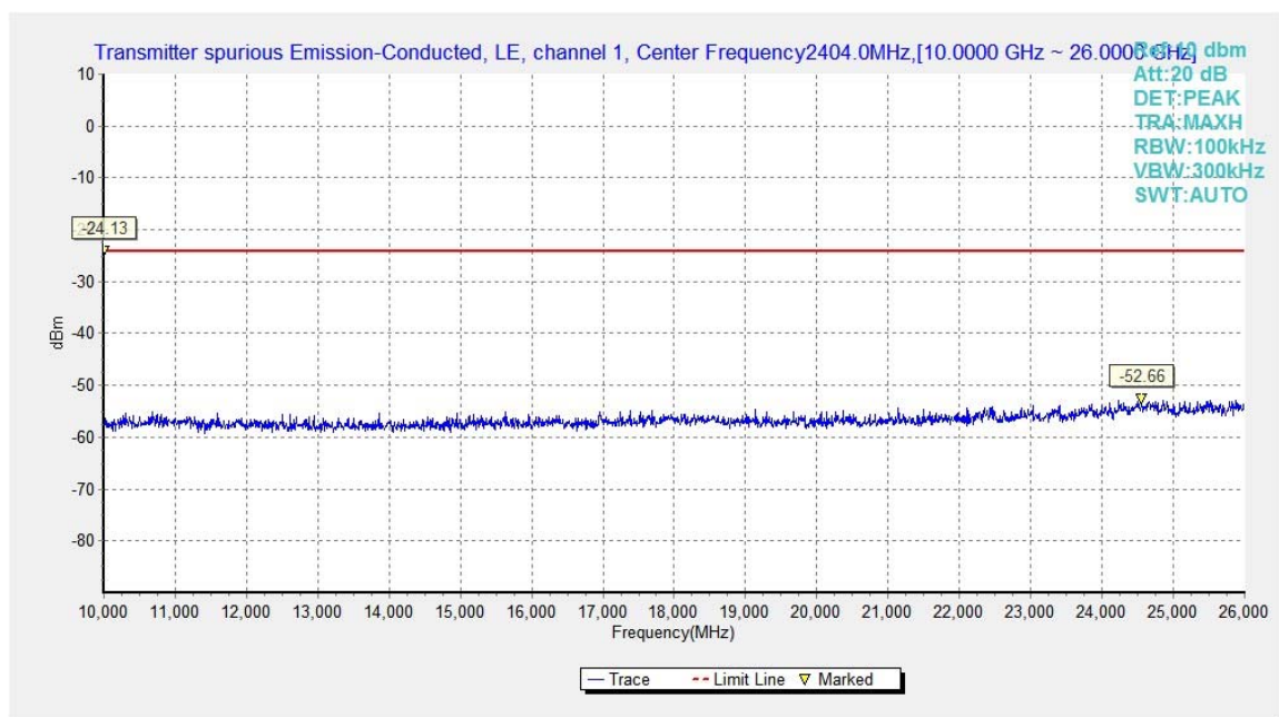
Fig.9. Transmitter Spurious Emission - Conducted: GFSK, 2404 MHz, 10GHz - 26GHz
