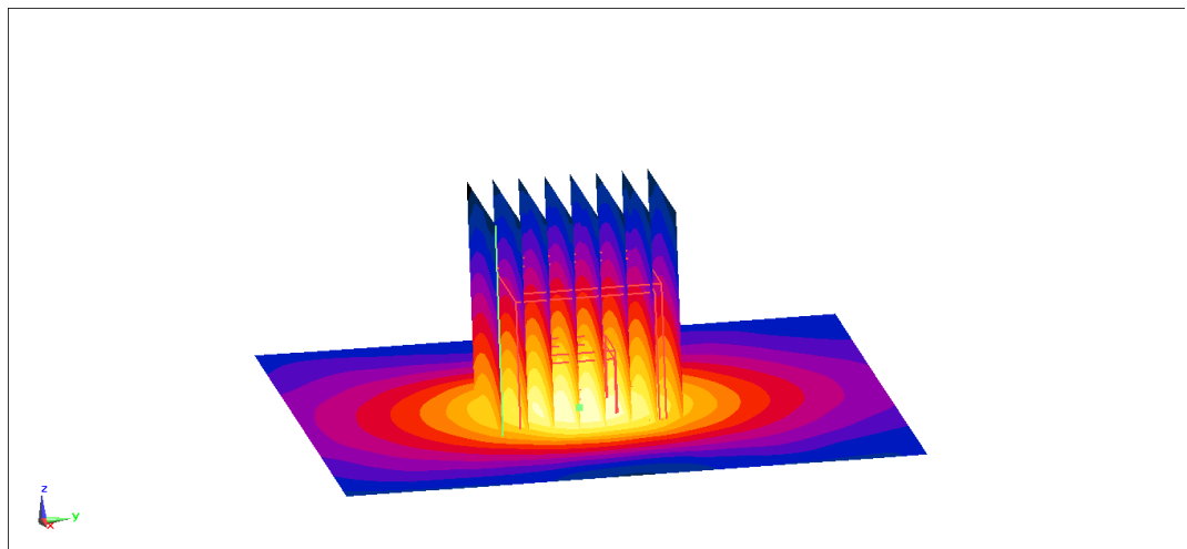
Fig.B.11 validation 3700 MHz 250mW
