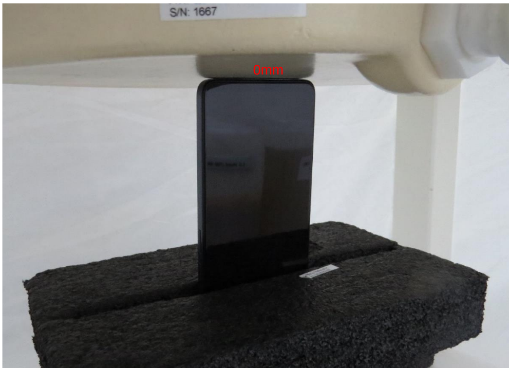
Picture 20: Bottom Edge, the distance from EUT to the bottom of the Phantom is 0mm
