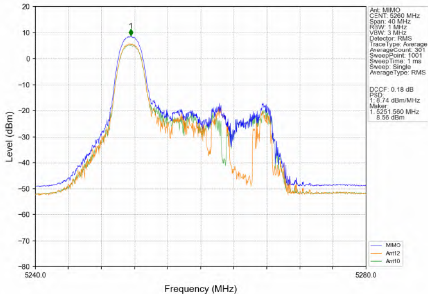
802.11ax(HEW20)_LCH_5260MHz_RU26_Left_MIMO_NTNV
