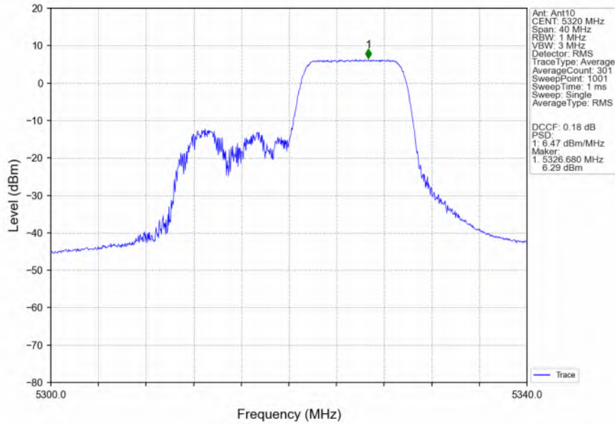
802.11ax(HEW20)_HCH_5320MHz_RU106_Right_MIMO_NTNV
