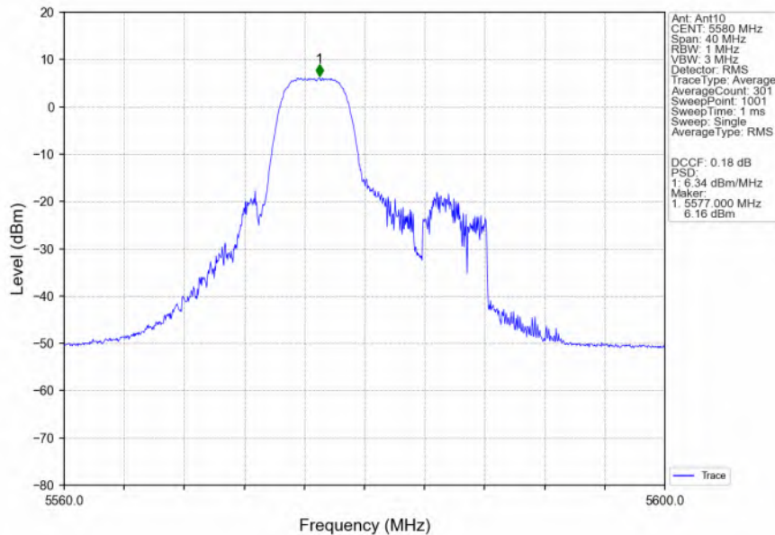
802.11ax(HEW20)_MCH_5580MHz_RU52_Mid_Ant10_NTNV
