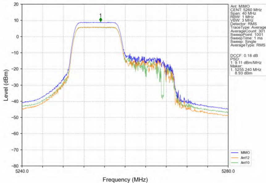
802.11ax(HEW20)_LCH_5260MHz_RU106_Left_MIMO_NTNV
