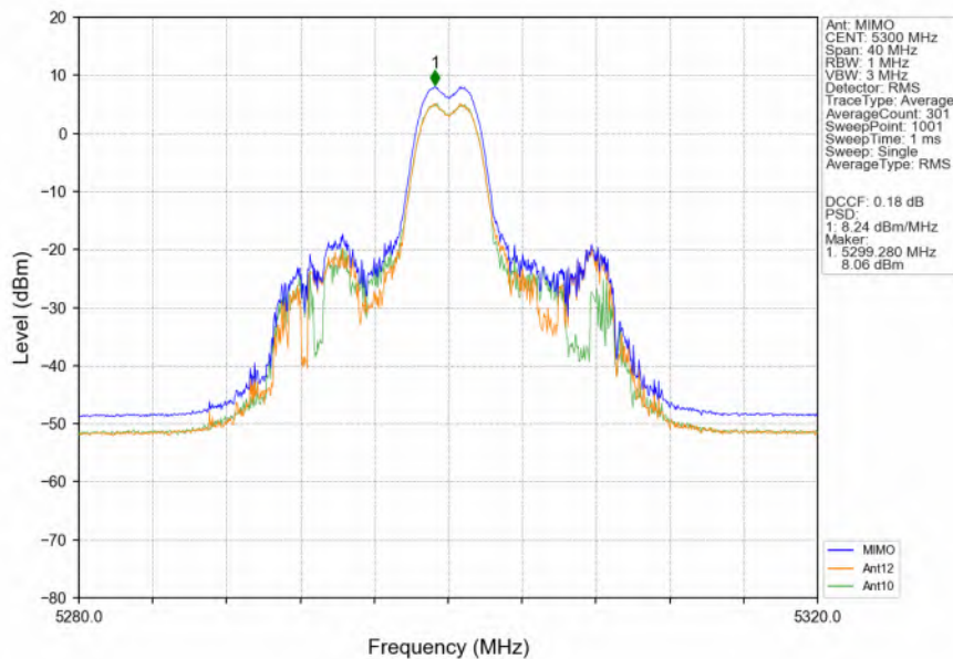
802.11ax(HEW20)_MCH_5300MHz_RU26_Mid_MIMO_NTNV
