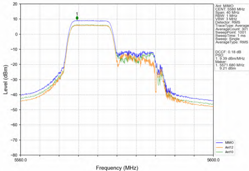
802.11ax(HEW20)_MCH_5580MHz_RU106_Left_MIMO_NTNV
