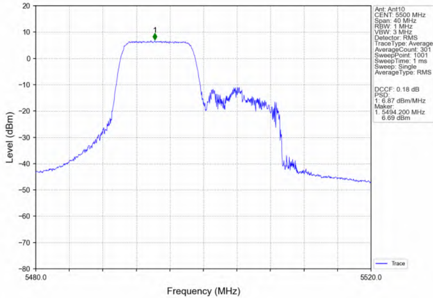
802.11ax(HEW20)_LCH_5500MHz_RU106_Left_MIMO_NTNV
