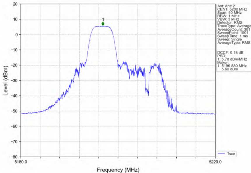
802.11ax(HEW20)_MCH_5200MHz_RU26_Mid_Ant12_NTNV
