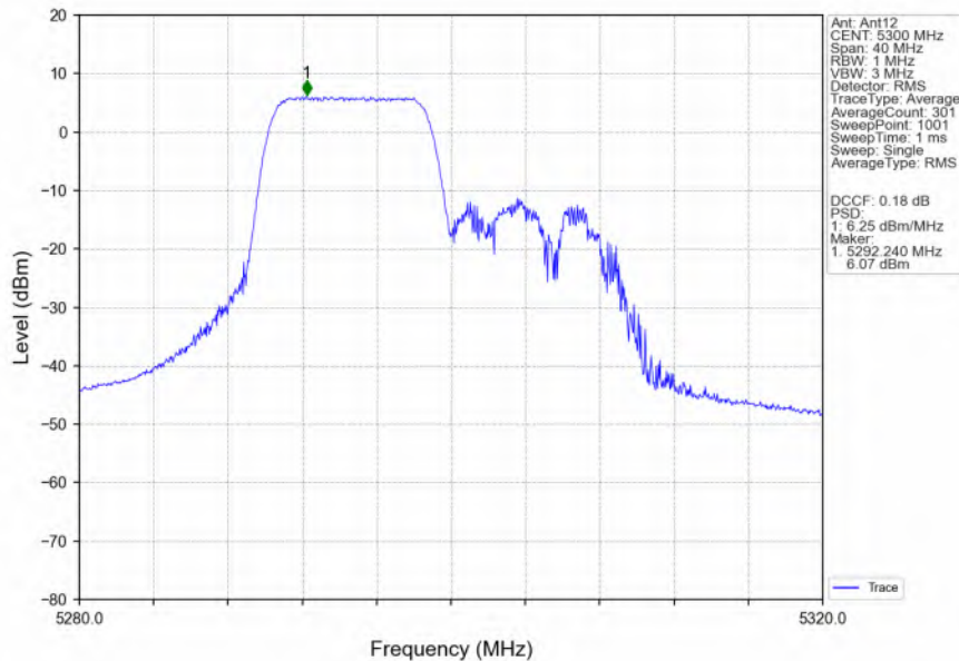
802.11ax(HEW20)_MCH_5300MHz_RU106_Left_Ant12_NTNV
