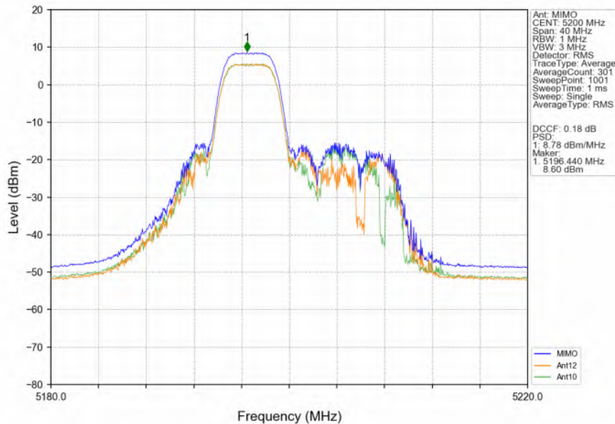
802.11ax(HEW20)_MCH_5200MHz_RU26_Mid_MIMO_NTNV
