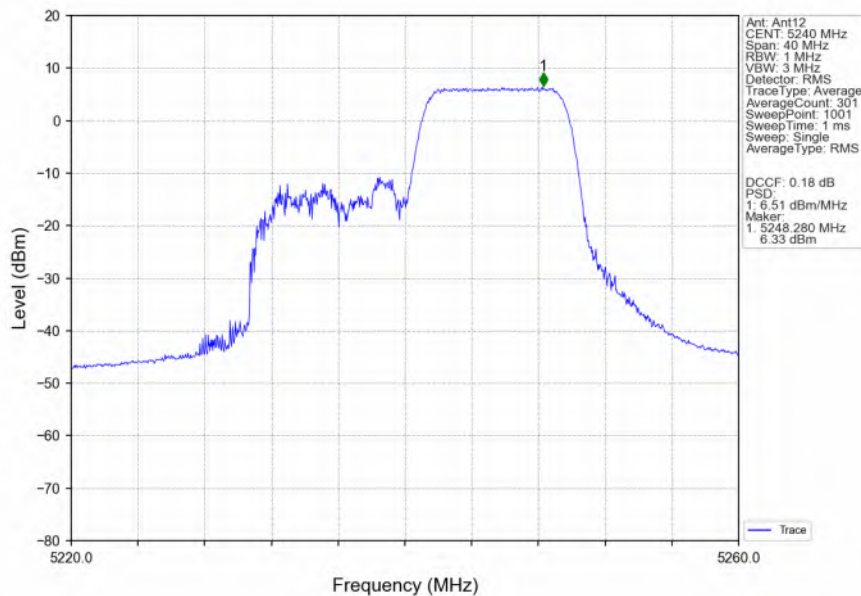
802.11ax(HEW20)_HCH_5240MHz_RU106_Right_Ant12_NTNV
