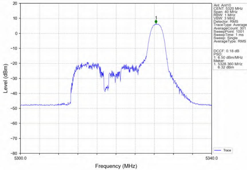
802.11ax(HEW20)_HCH_5320MHz_RU26_Right_MIMO_NTNV
