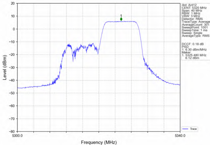
802.11ax(HEW20)_HCH_5320MHz_RU106_Right_Ant12_NTNV
