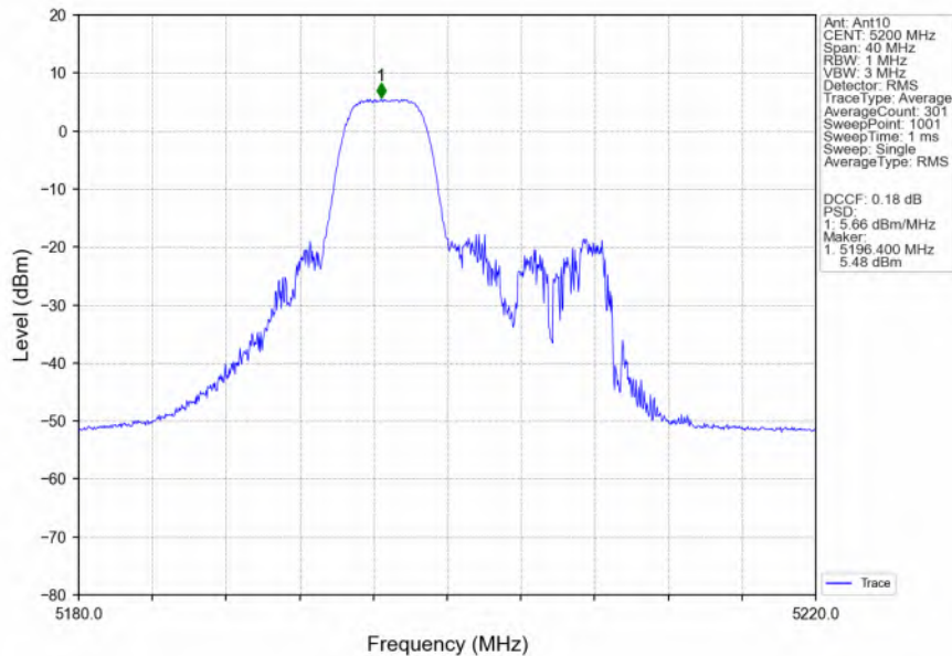
802.11ax(HEW20)_MCH_5200MHz_RU52_Mid_Ant10_NTNV
