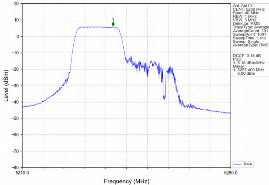
802.11ax(HEW20)_LCH_5260MHz_RU106_Left_MIMO_NTNV
