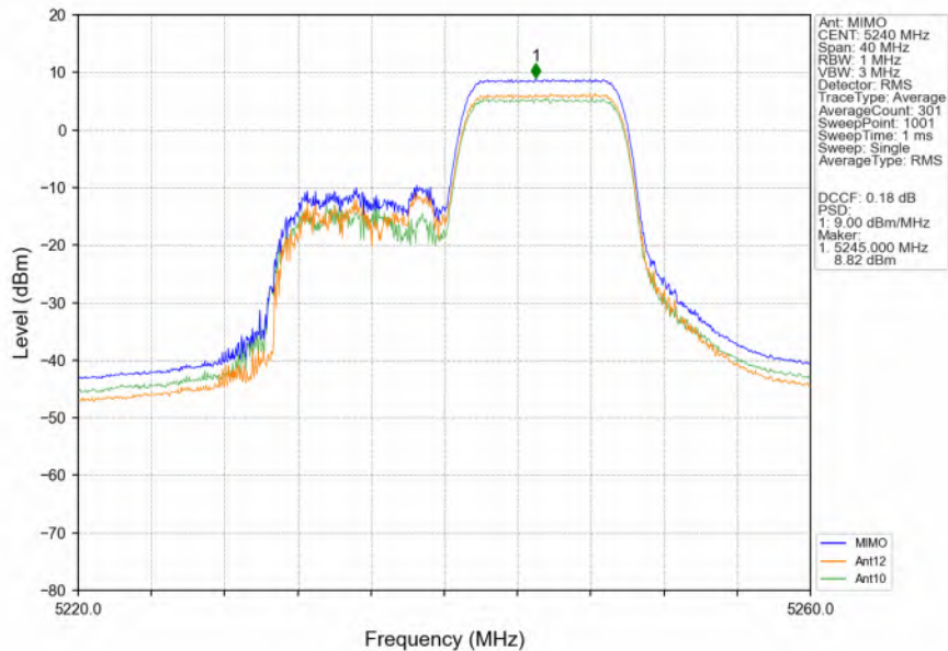
802.11ax(HEW20)_HCH_5240MHz_RU106_Right_MIMO_NTNV
