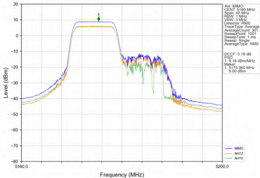
802.11ax(HEW20)_LCH_5180MHz_RU106_Left_MIMO_NTNV
