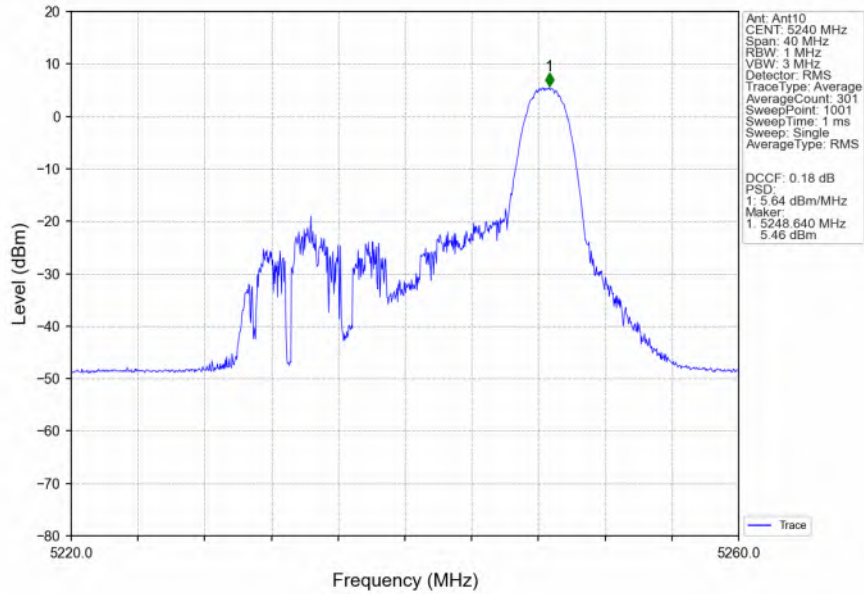
802.11ax(HEW20)_HCH_5240MHz_RU26_Right_MIMO_NTNV
