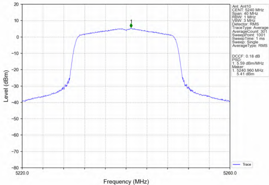
802.11ax(HEW20)_HCH_5240MHz_RU242_Left_Ant10_NTNV
