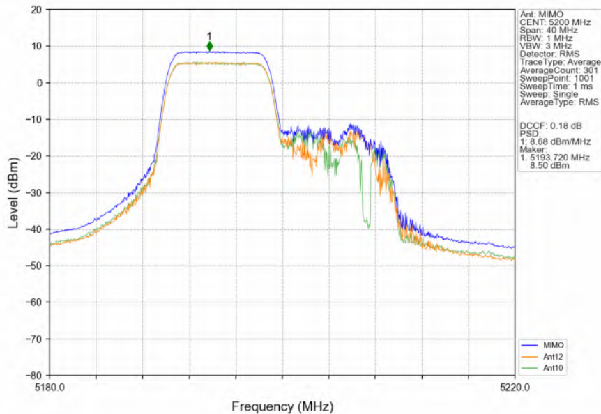
802.11ax(HEW20)_MCH_5200MHz_RU106_Left_MIMO_NTNV
