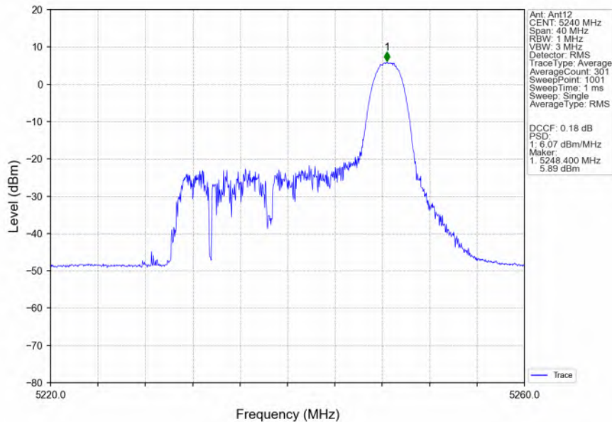
802.11ax(HEW20)_HCH_5240MHz_RU26_Right_Ant12_NTNV
