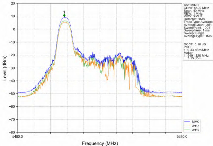
802.11ax(HEW20)_LCH_5500MHz_RU26_Left_MIMO_NTNV
