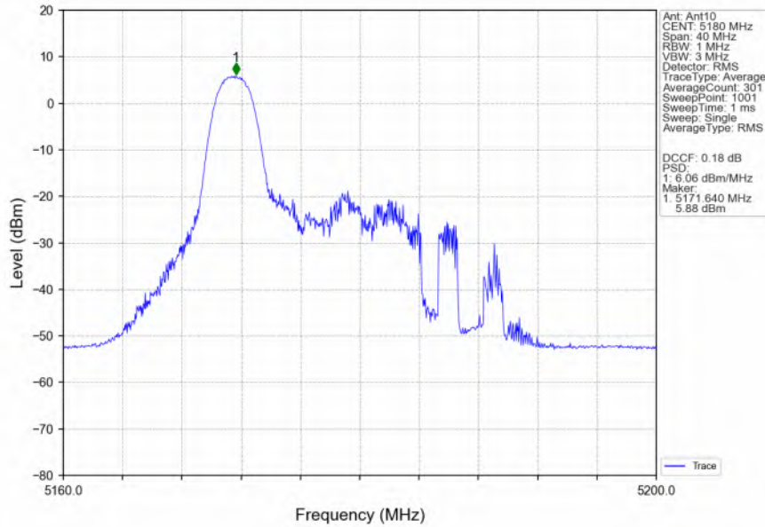
802.11ax(HEW20)_LCH_5180MHz_RU26_Left_MIMO_NTNV
