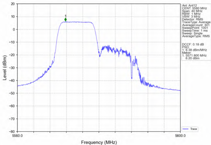
802.11ax(HEW20)_MCH_5580MHz_RU106_Left_Ant12_NTNV
