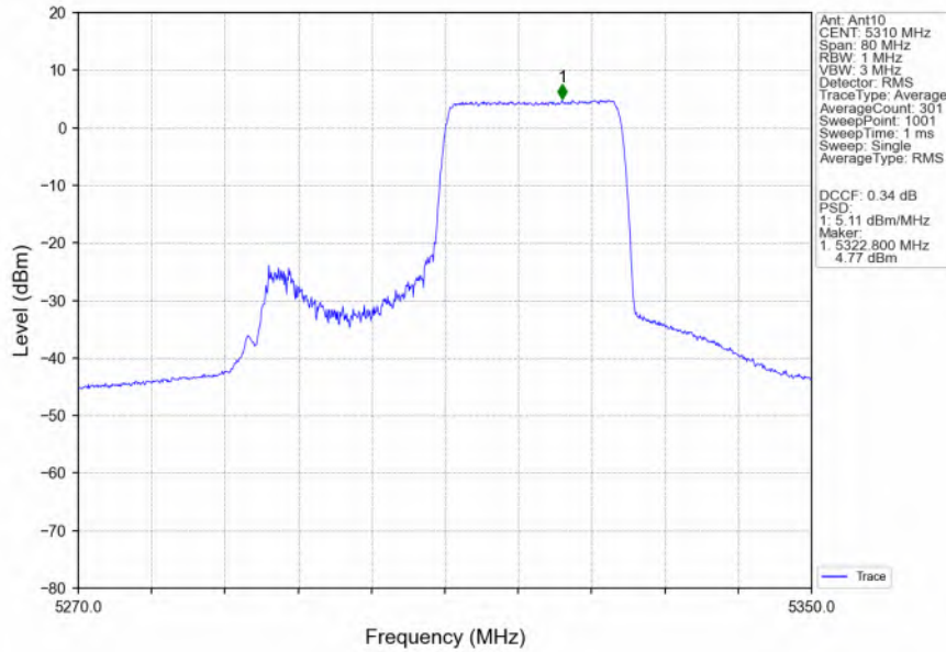
802.11ax(HEW40)_HCH_5310MHz_RU242_Right_MIMO_NTNV
