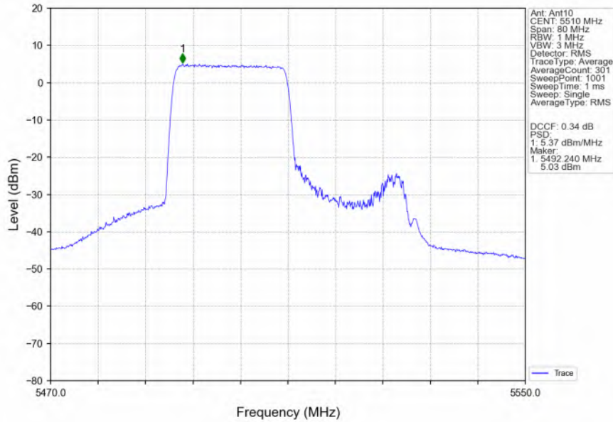
802.11ax(HEW40)_LCH_5510MHz_RU242_Left_MIMO_NTNV
