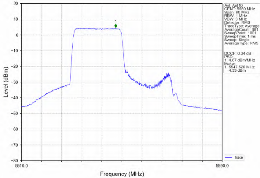
802.11ax(HEW40)_MCH_5550MHz_RU242_Left_MIMO_NTNV
