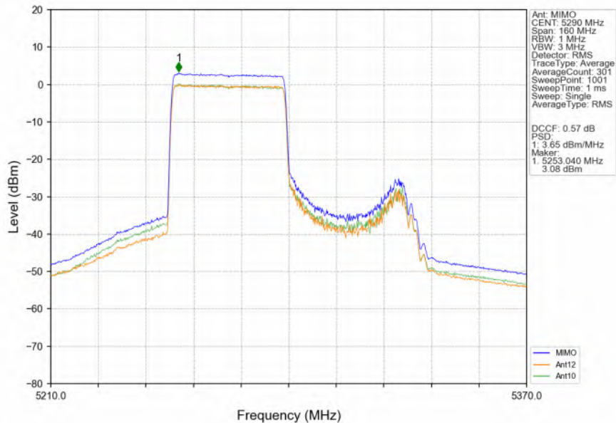
802.11ax(HEW80)_MCH_5290MHz_RU484_Left_MIMO_NTNV
