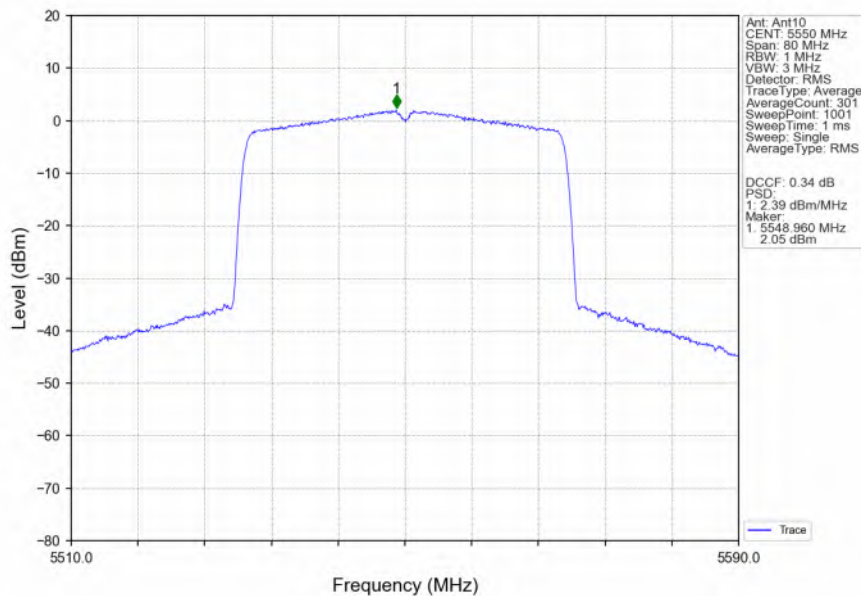
802.11ax(HEW40)_MCH_5550MHz_RU484_Left_Ant10_NTNV
