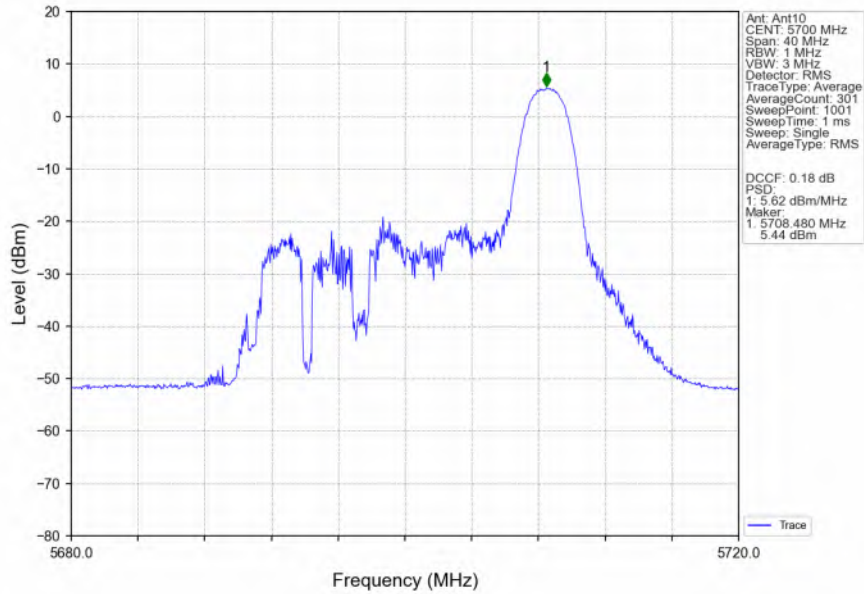
802.11ax(HEW20)_HCH_5700MHz_RU26_Right_MIMO_NTNV
