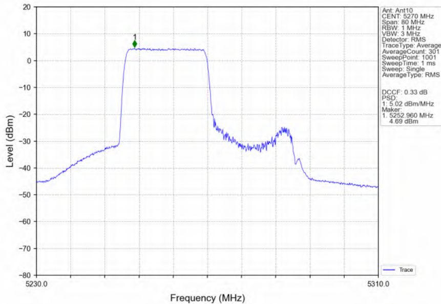
802.11ax(HEW40)_LCH_5270MHz_RU242_Left_MIMO_NTNV
