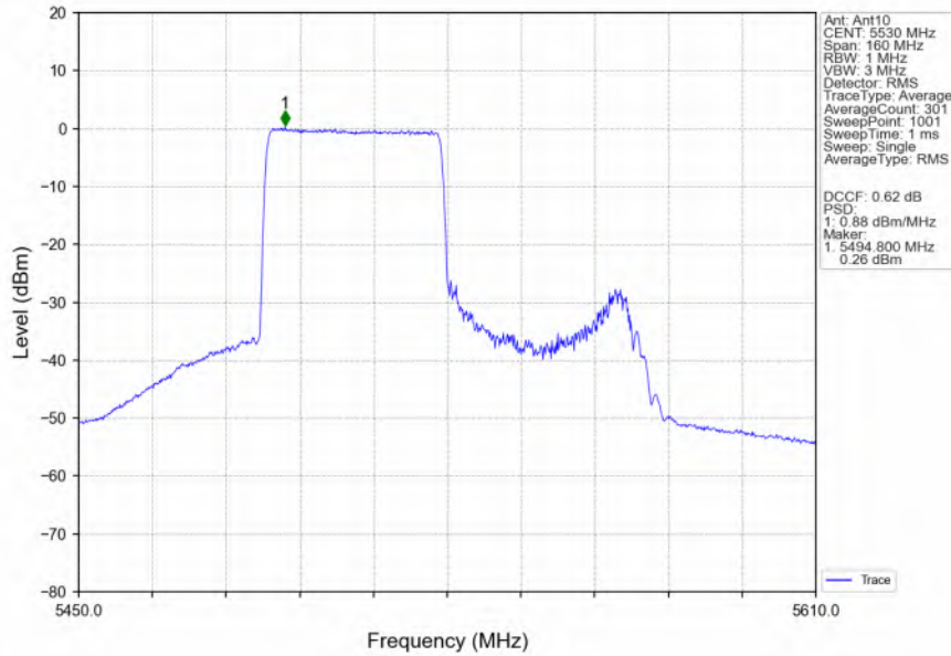
802.11ax(HEW80)_LCH_5530MHz_RU484_Left_MIMO_NTNV
