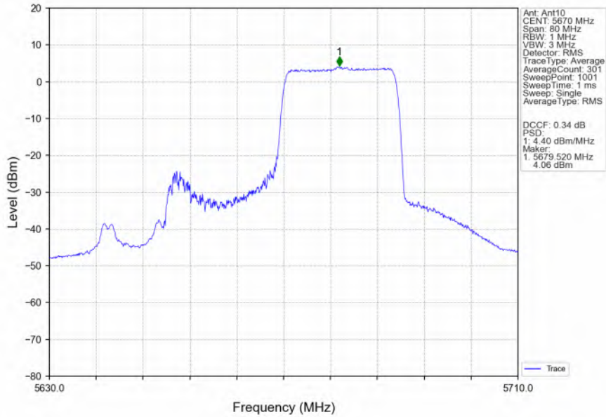
802.11ax(HEW40)_HCH_5670MHz_RU242_Right_MIMO_NTNV
