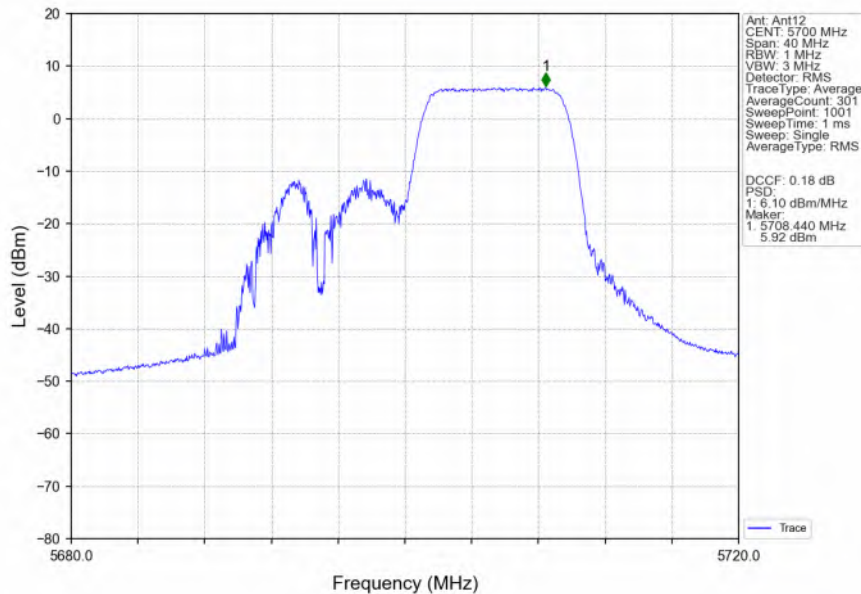
802.11ax(HEW20)_HCH_5700MHz_RU106_Right_Ant12_NTNV
