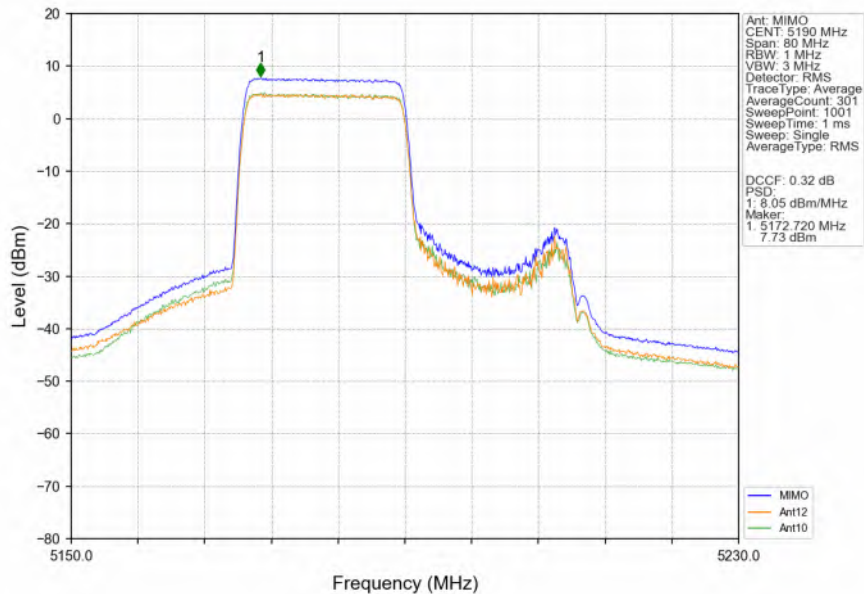
802.11ax(HEW40)_LCH_5190MHz_RU242_Left_MIMO_NTNV
