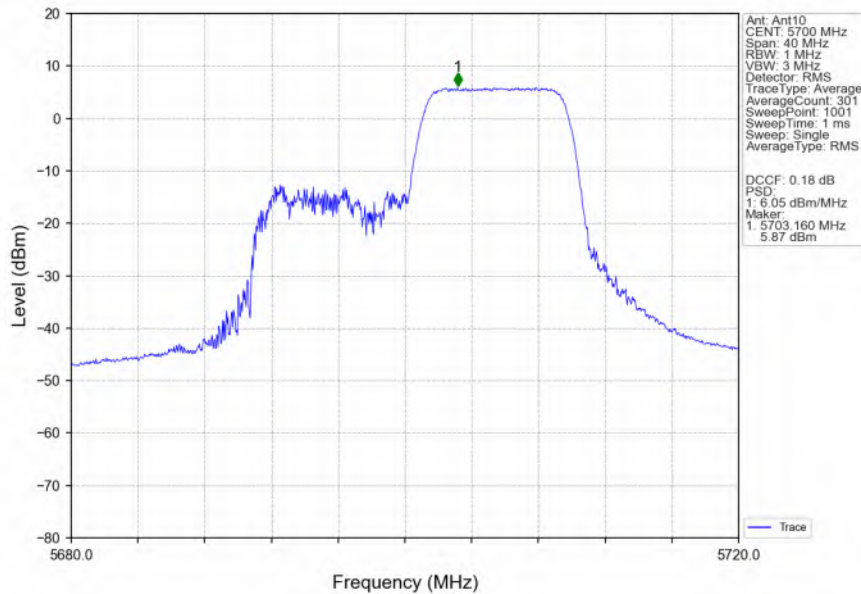
802.11ax(HEW20)_HCH_5700MHz_RU106_Right_MIMO_NTNV
