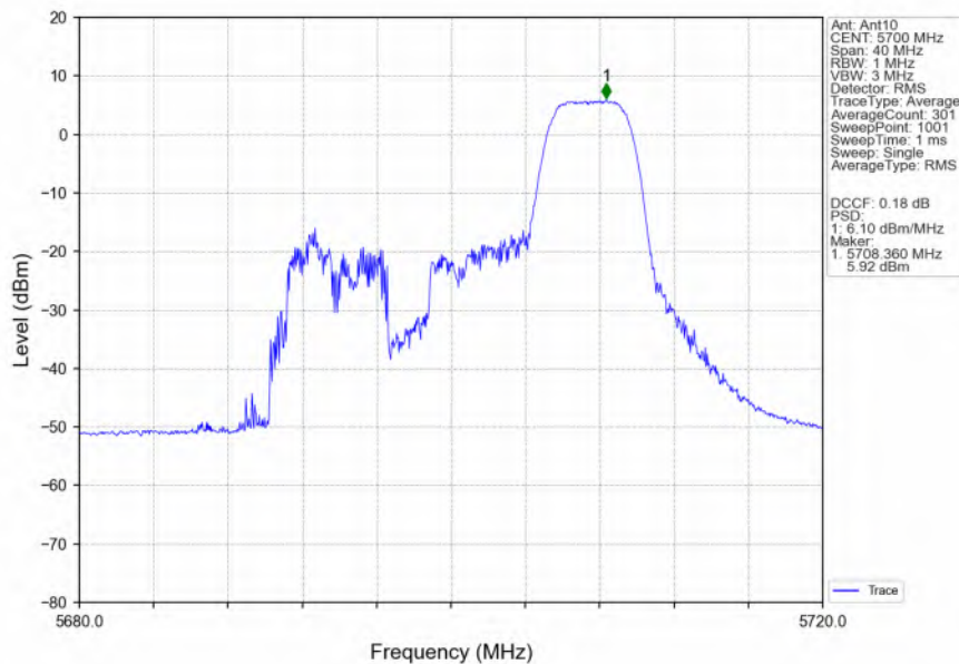
802.11ax(HEW20)_HCH_5700MHz_RU52_Right_Ant10_NTNV
