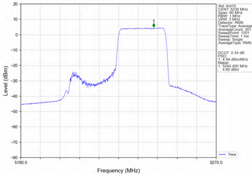
802.11ax(HEW40)_HCH_5230MHz_RU242_Right_MIMO_NTNV
