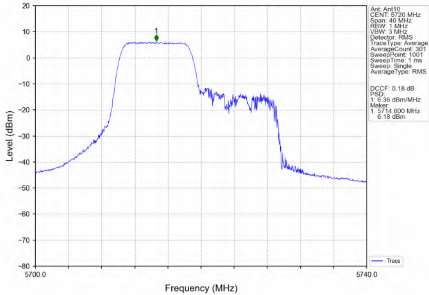
802.11ax(HEW20)_HCH_5720MHz_RU106_Left_MIMO_NTNV
