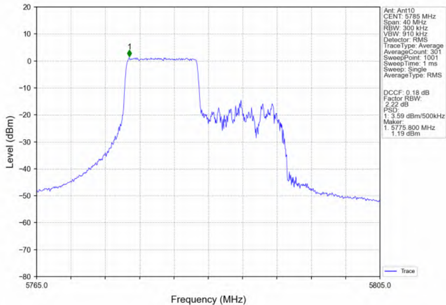
802.11ax(HEW20)_MCH_5785MHz_RU106_Left_Ant10_NTNV
