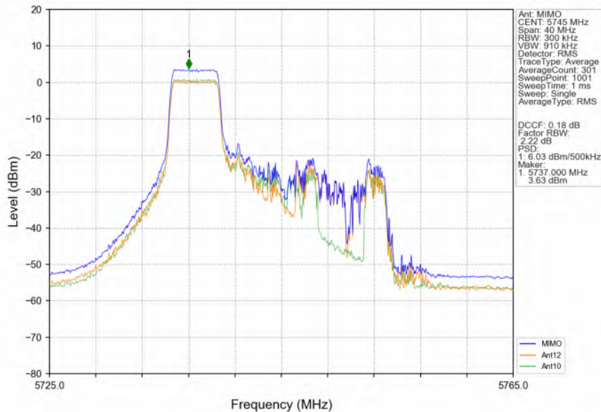
802.11ax(HEW20)_LCH_5745MHz_RU52_Left_MIMO_NTNV
