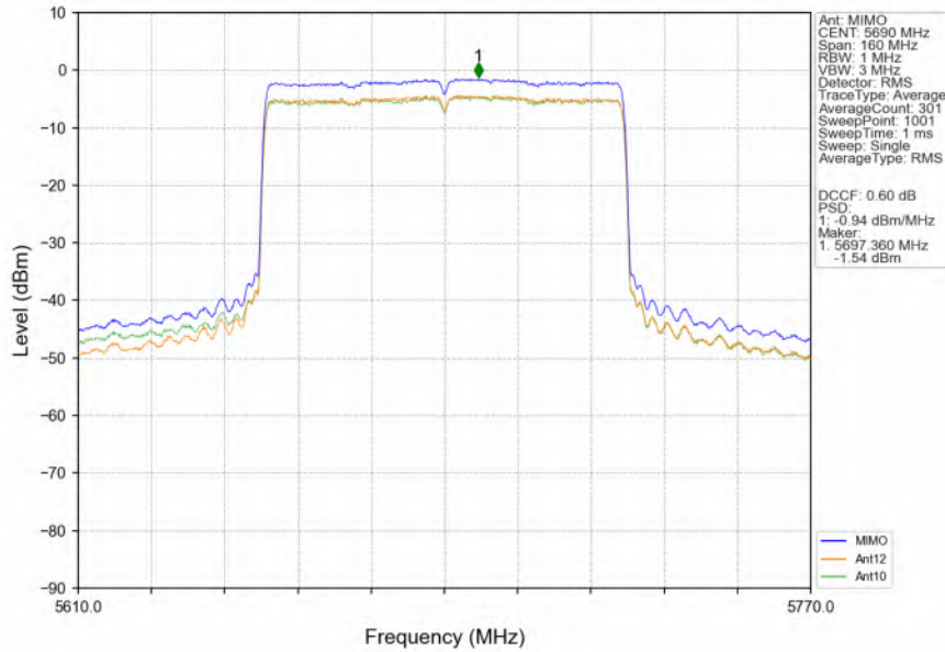
802.11ax(HEW80)_HCH_5690MHz_RU996_Left_MIMO_NTNV
