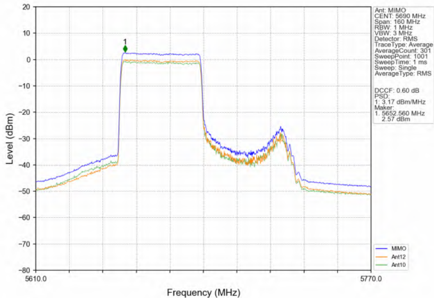
802.11ax(HEW80)_HCH_5690MHz_RU484_Left_MIMO_NTNV
