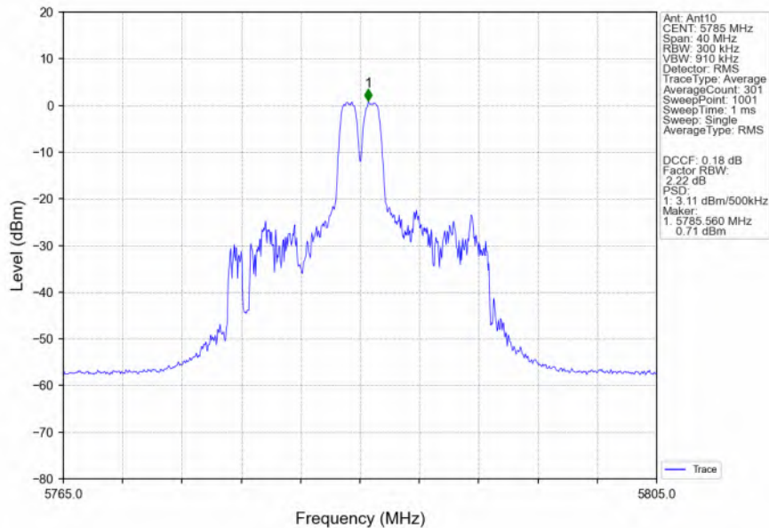
802.11ax(HEW20)_MCH_5785MHz_RU26_Mid_Ant10_NTNV
