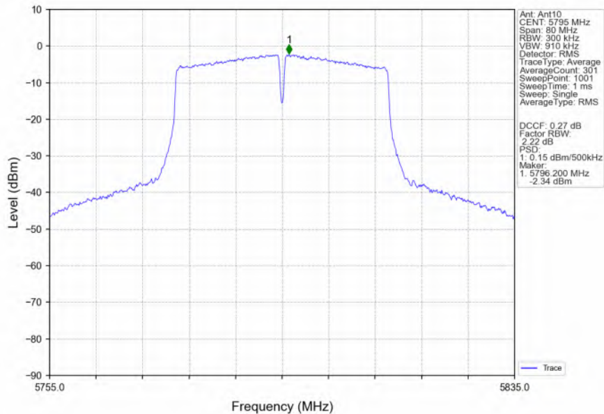
802.11ac(VHT40)_HCH_5795MHz_Ant10_NTNV
