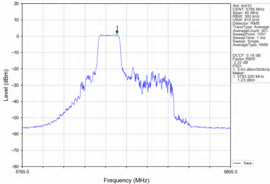
802.11ax(HEW20)_MCH_5785MHz_RU52_Mid_MIMO_NTNV
