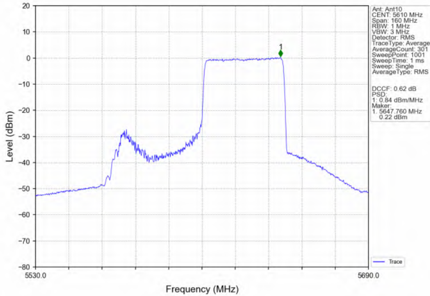
802.11ax(HEW80)_HCH_5610MHz_RU484_Right_MIMO_NTNV
