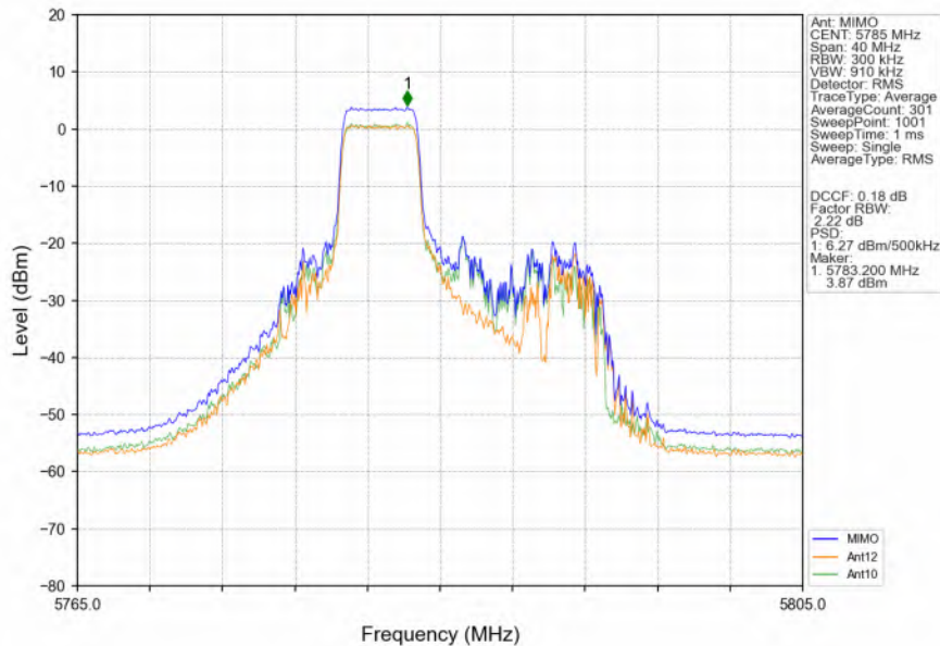
802.11ax(HEW20)_MCH_5785MHz_RU52_Mid_MIMO_NTNV
