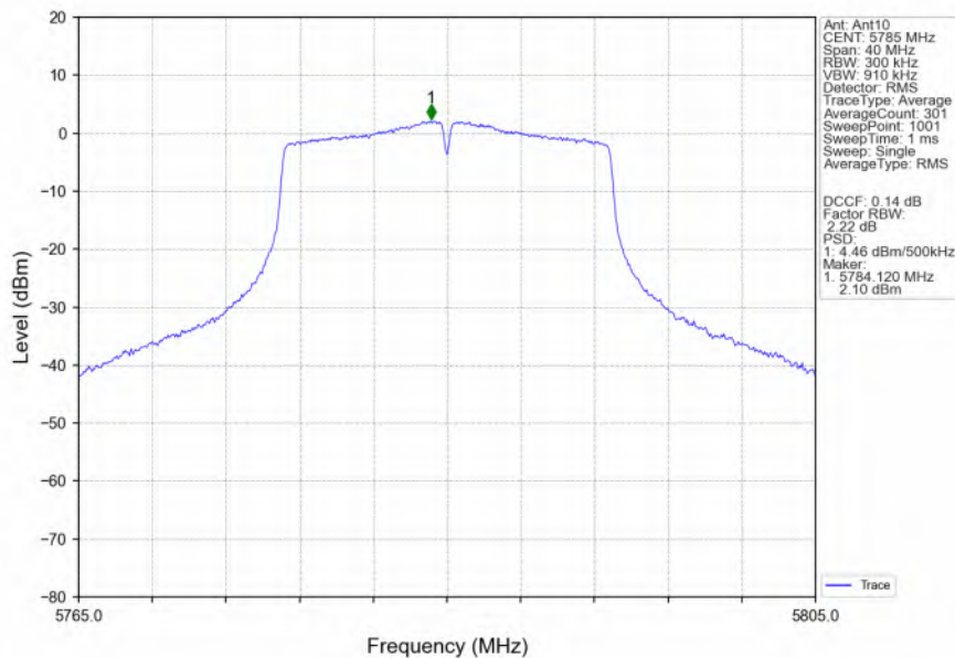
802.11ac(VHT20)_MCH_5785MHz_Ant10_NTNV
