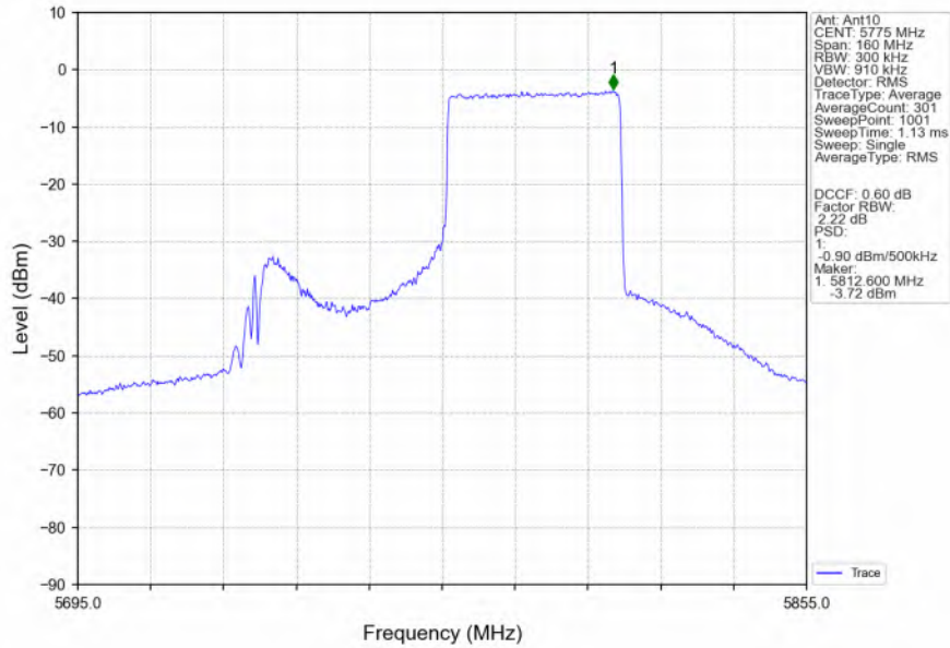
802.11ax(HEW80)_MCH_5775MHz_RU484_Right_MIMO_NTNV
