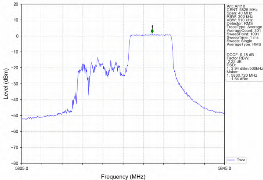
802.11ax(HEW20)_HCH_5825MHz_RU106_Right_Ant10_NTNV
