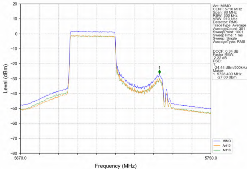
802.11ax(HEW40)_HCH_5710MHz_RU242_Left_MIMO_NTNV
