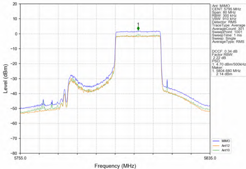
802.11ax(HEW40)_HCH_5795MHz_RU242_Right_MIMO_NTNV
