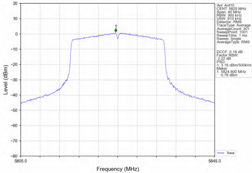
802.11ax(HEW20)_HCH_5825MHz_RU242_Left_MIMO_NTNV
