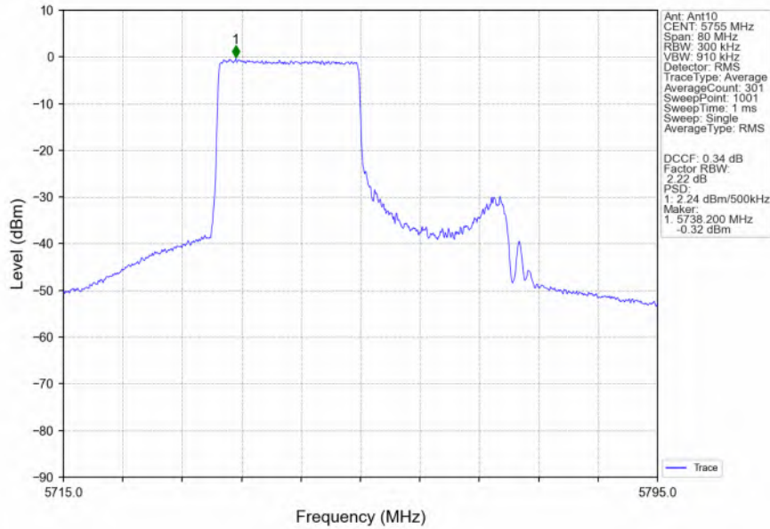
802.11ax(HEW40)_LCH_5755MHz_RU242_Left_MIMO_NTNV
