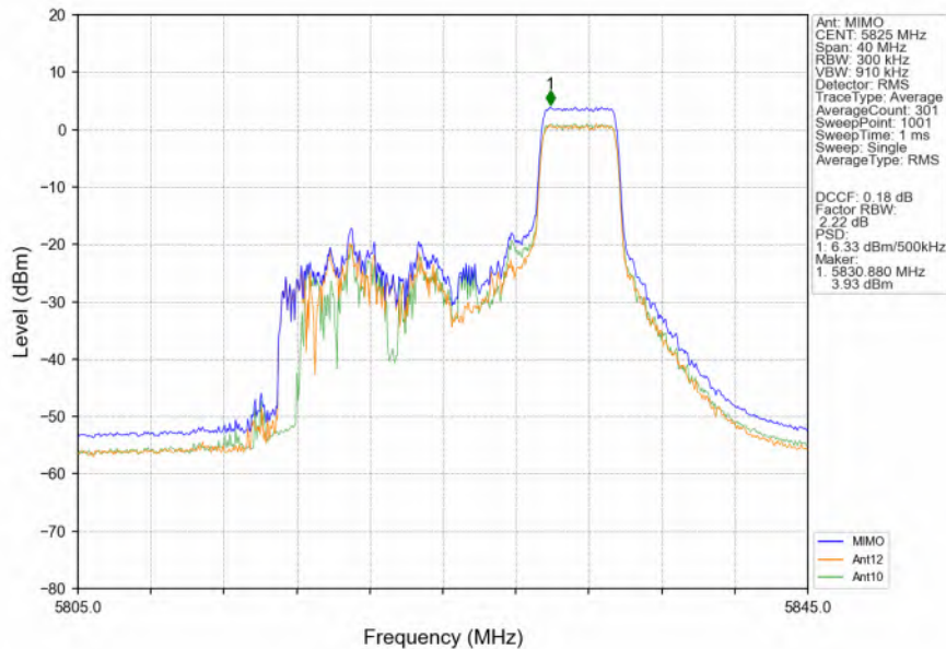
802.11ax(HEW20)_HCH_5825MHz_RU52_Right_MIMO_NTNV
