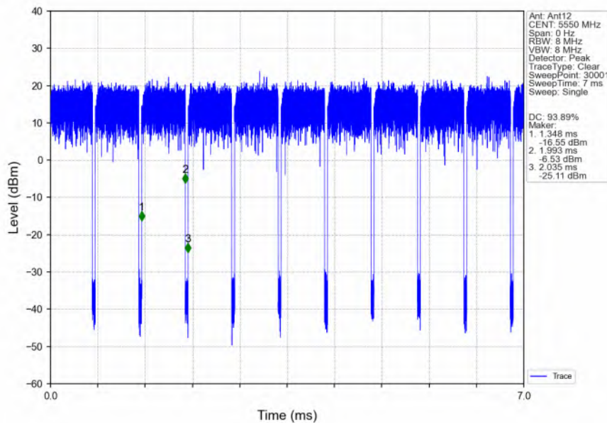
802.11n(HT40)_MCH_5550MHz_Ant12_NTNV
