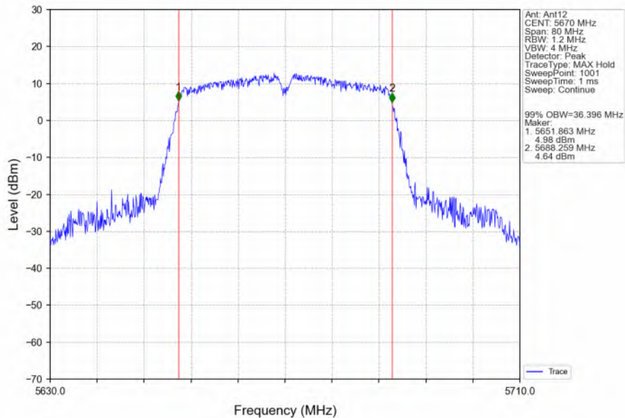
802.11ac(VHT40)_HCH_5670MHz_Ant12_NTNV
