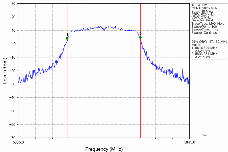
802.11a_HCH_5825MHz_Ant12_NTNV
