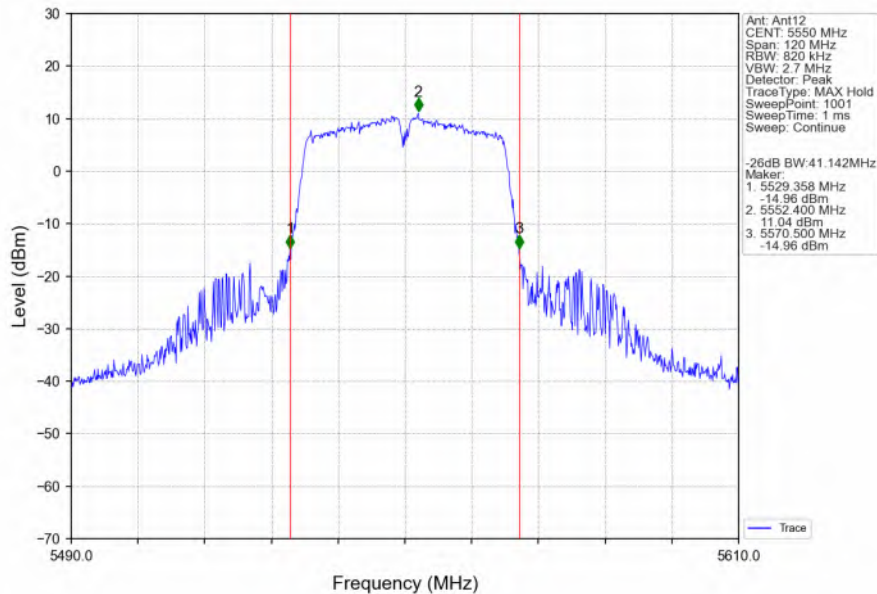
802.11n(HT40)_MCH_5550MHz_Ant12_NTNV
